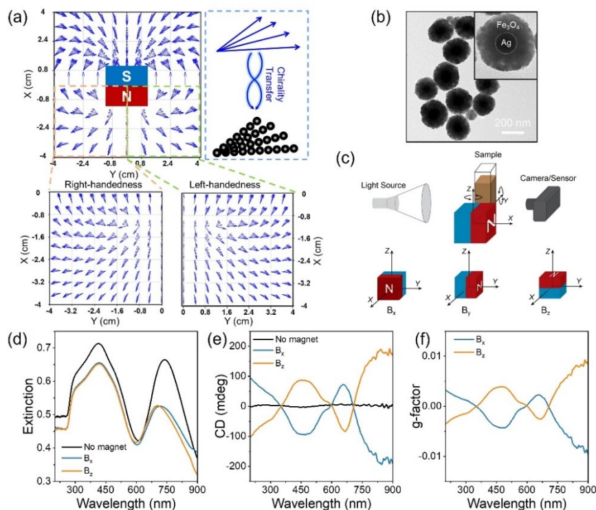
Figure 1. (a) Simulation of the chiral field distribution from a cubic permanent magnet and schematic illustration of the chirality transfer from chiral magnetic field to magnetic nanoparticle assembly. (b) TEM image of \text{Ag}@\text{Fe}_3\text{O}_4 hybrid nanoparticles. (c) Schematic illustration of the setup for measuring the extinction and CD spectrum of particle dispersion under a chiral magnetic field. (d-f) Extinction (d), CD (e), and the corresponding g-factor (f) spectra of the \text{Ag}@\text{Fe}_3\text{O}_4 nanoparticle dispersion without a magnetic field or under a field along the X- and Z-axes.
