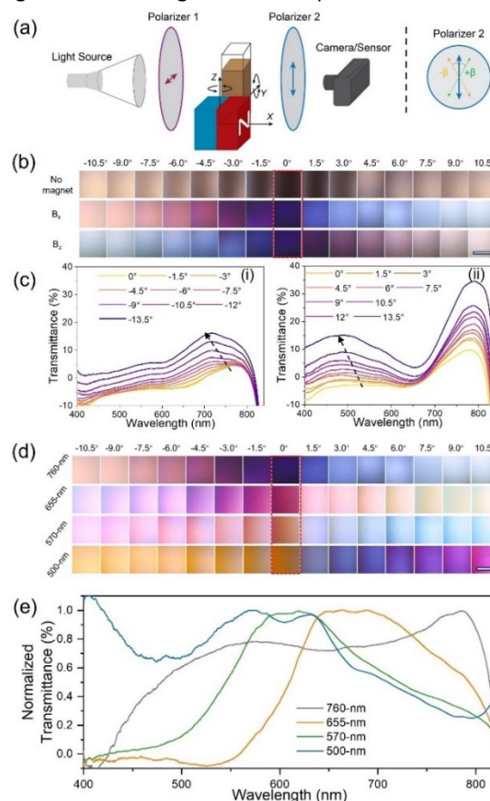
Figure 4. (a) Schematic illustration of ORD measurement setup. (b) ORD images of Ag@Fe 3 O 4 nanoparticle dispersion under no magnetic field or B_x and B_z fields. (c) The transmission spectra of the nanoparticle dispersion under B_x with varying negative (i) and positive (ii) \beta . (d) ORD images of Ag@Fe 3 O 4 nanoparticles with 760, 655, 570, and 500 nm extinction peaks under B_x with varying \beta from -10.5 to 10.5^\circ . (e) Corresponding transmission spectra of the sample in (d) at \beta=0^\circ . All the digital images in (b) and (d) share the same scale bar of 1 mm.
