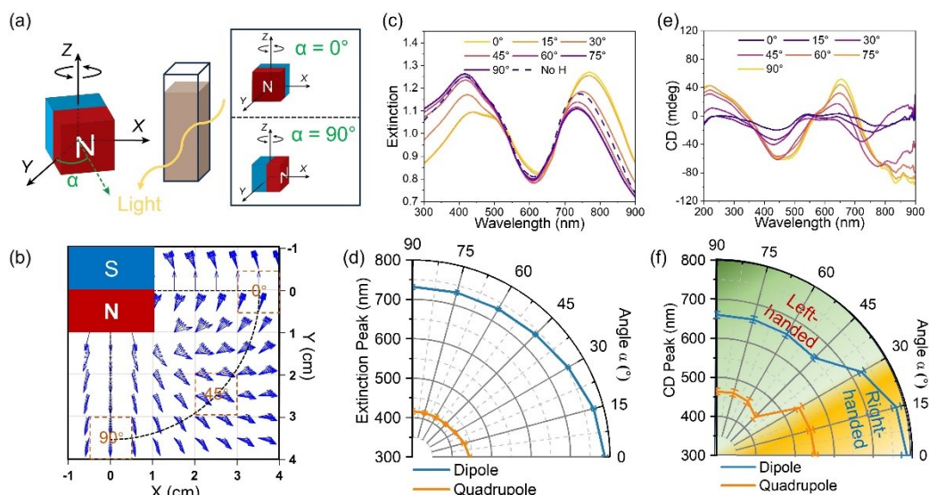
Figure 2. (a) Scheme illustrating the field rotation of a cubic magnet along the Z-axis within the XY-plane. (b) Simulation of magnetic field distribution as the north pole rotated from the X-axis (90°) to the Y-axis (0°). (c, d) Extinction spectra and the corresponding dipole and quadrupole peak shifts of the Ag@Fe 3 O 4 nanoparticle assemblies upon varying the field from B_x to B_y . (e, f) CD spectra and the corresponding dipole and quadrupole peak shifts of the assemblies upon varying the field from B_x to B_y .
