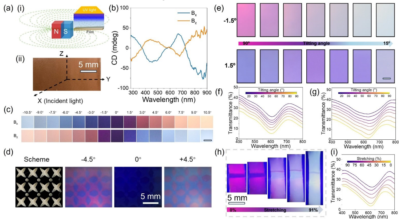
Figure 5. (a) Scheme illustrating fixing the plasmonic chiral superstructures in a polymer film (i) and photo of the assembled chiral film (ii). (b) CD spectra of the chiral film with left- and right-handedness. (c) ORD images of the left- and right-handed chiral film under varying \beta from -10.5 to 10.5^\circ . (d) Scheme and ORD images of a chiral film pattern with left-handed chiral nanostructures in white regions and right-handed chiral nanostructures in black regions as \beta = 0 , and \pm 4.5^\circ . (e-g) ORD images of the chiral film as the angle between light direction and film varied from 90 to 15^\circ at \beta = \pm 1.5^\circ (e) and the corresponding transmission spectra at \beta = -1.5^\circ (f) and \beta = 1.5^\circ (g). (h, i) ORD images of the chiral film under stretching from 0 to 91\% as \beta = -1.5^\circ (h) and the corresponding transmission spectra (i). All the digital images in Figures (c) and (e) share the same scale bar of 1 mm.
