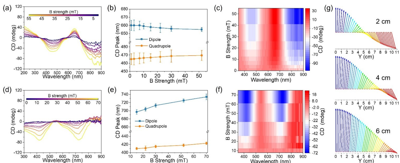
Figure 3. (a-f) CD spectra (a, d), the corresponding dipole and quadrupole peak shifts (b, e), and the peak intensity changes (c, f) of Ag@Fe 3 O 4 nanoparticle assembly under B_x and B_y with varying strength. (g) Simulated magnetic field vector rotation along the Y-axis under different distances (2, 4, 6 cm) along the X-axis from the magnet, showing chirality decreases with increasing separation distance.
