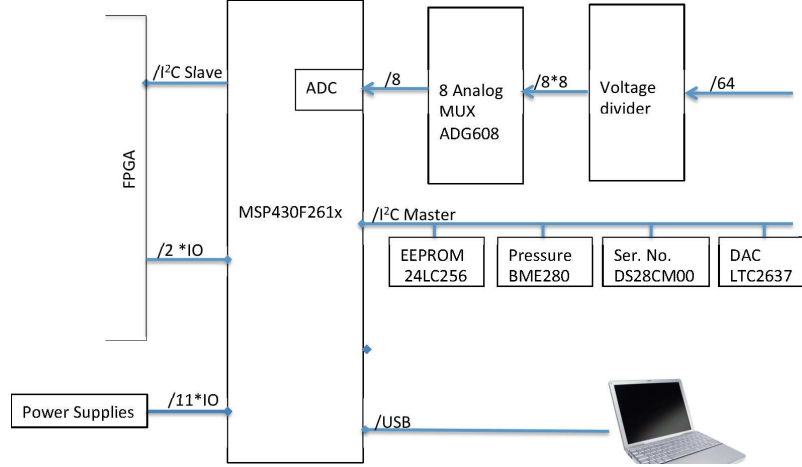
Figure 5. Block diagram of the slow-control system.
