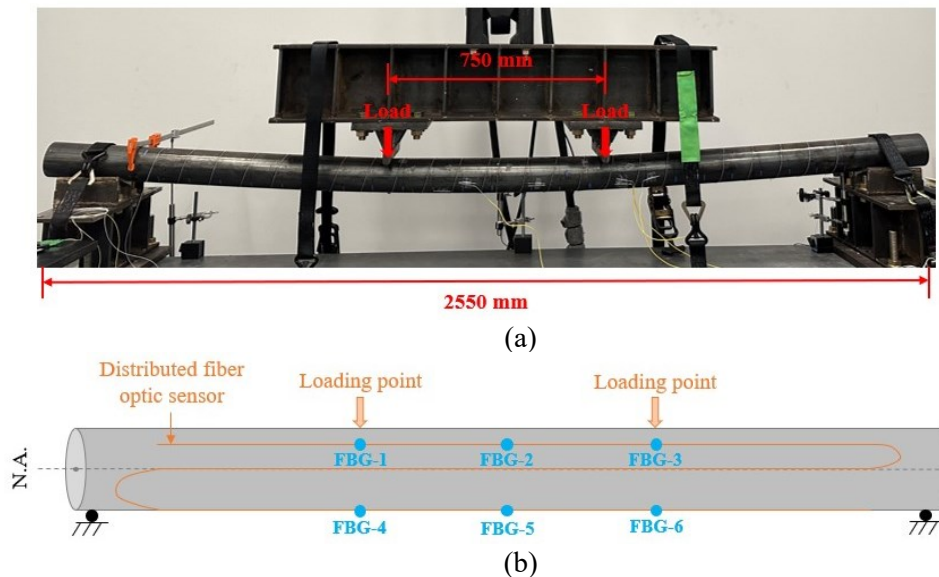
Fig. 2 Experimental test set-up: (a) photograph of the four-point bending test; (b) deployment of FBG sensors on the pipe-elevation view.
