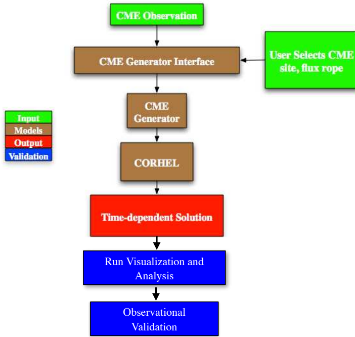
Figure 1. Framework diagram for CORHEL-CME.
