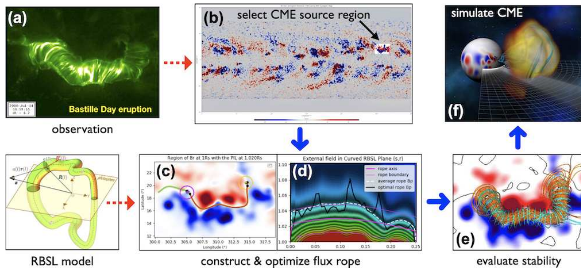
Figure 2. Main steps of modeling a CME with CORHEL-CME. See text for details.
