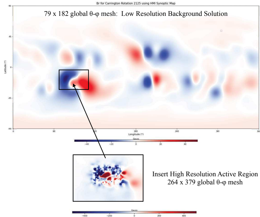
Figure 5. Latitude-longitude map of B_r boundary for low resolution background simulation of the ambient corona around the time of the July 12, 2012 CME, together with the high resolution active region that would be inserted and re-meshed for a CORHEL-CME simulation.
