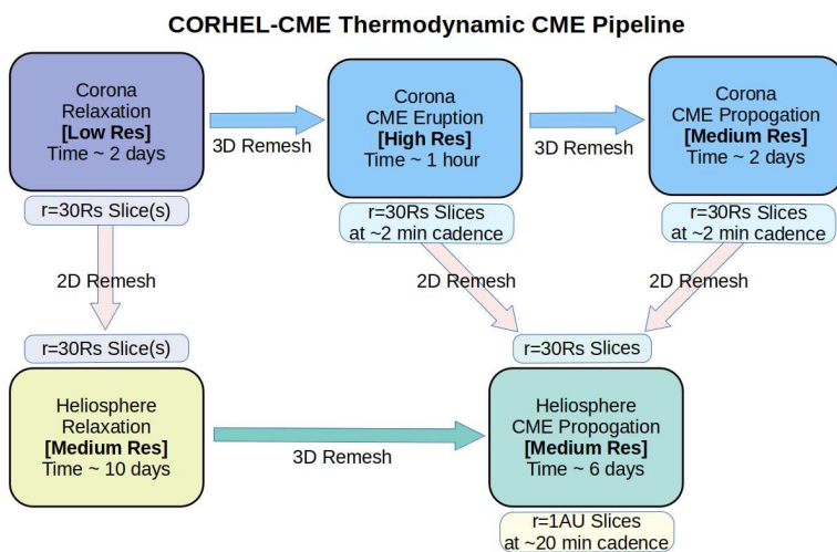
Figure 4. Flow chart showing the run pipeline for modeling a single Sun-to-1 AU CME in the corona and inner heliosphere. This corresponds to STEP 3 and STEP 4 in Figure 3.
