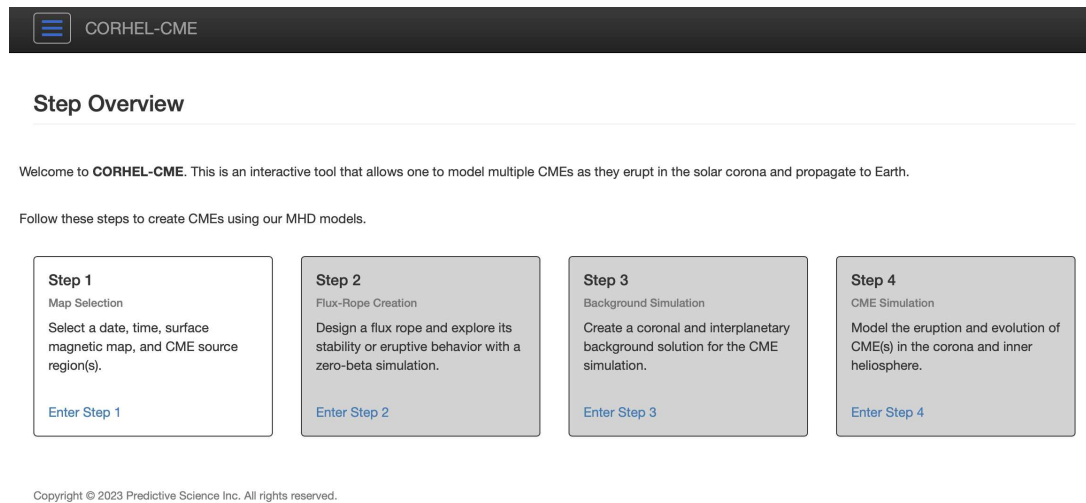
Figure 3. Navigation page of the CORHEL-CME web interface. The user is guided through the process via various steps that include magnetogram and source-region selection (Step 1), RBSL flux-rope configuration (Step 2), Set-up of background models (Step 3) and final CME simulation (Step 4).
