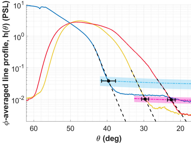
FIG. 3. The \phi -averaged line profile, h(\theta) (see text), for data in Figs. 2(a)–2(c), represented by red (far right), yellow, and dark blue (far left) curves, respectively. The dashed lines indicate exponential fits used to determine \theta_c . The dot-dashed magenta (blue) curve indicates the single-electron PSL level for the BAS-SR (BAS-MS) plates used for Figs. 2(a) and 2(b) [Fig. 2(c)] and the shaded regions are the estimated uncertainties in these levels based on measurements in Ref. [50]. The solid data points represent our best estimate of \theta_c and the associated uncertainty (see text).
