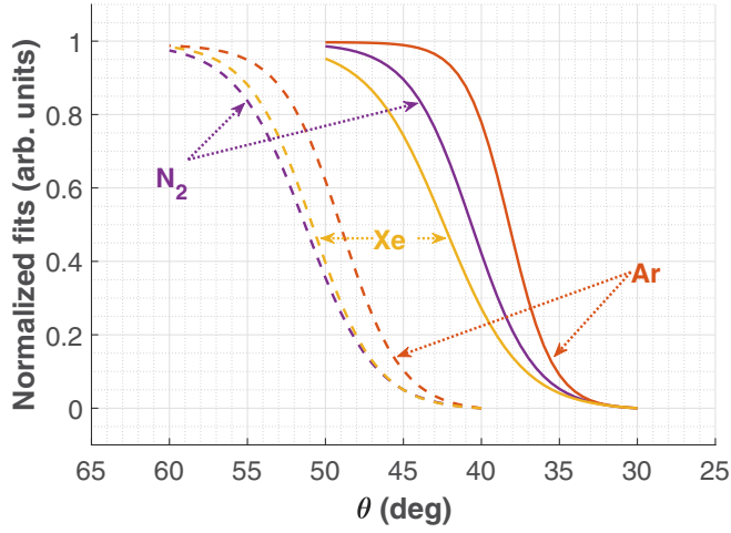
FIG. 5. Normalized and background subtracted sigmoid fits for the small-angle falloff of measurements performed with N_2 (violet), Ar (orange), and Xe (yellow). The solid (dashed) curves correspond to high (low) energy measurements.
