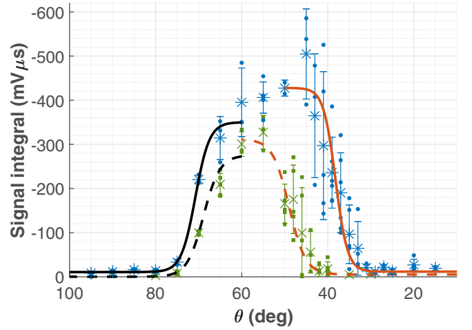
FIG. 4. Single-shot scintillation data captured with Ar gas for 15^\circ \leq \theta \leq 95^\circ with 26.7 J (blue dots) and 10.2 J (green squares) of laser energy on target for the experimental conditions detailed in Table II. The average high (low) energy data are displayed as “*” (“x”) along with their corresponding standard deviations. The solid (dashed) orange and black lines are sigmoid fits to the small and large angle falloff, respectively, for the high- (low-)energy measurement. The large angle threshold is set by the aluminum filters used to block the plethora of low-energy electrons.
