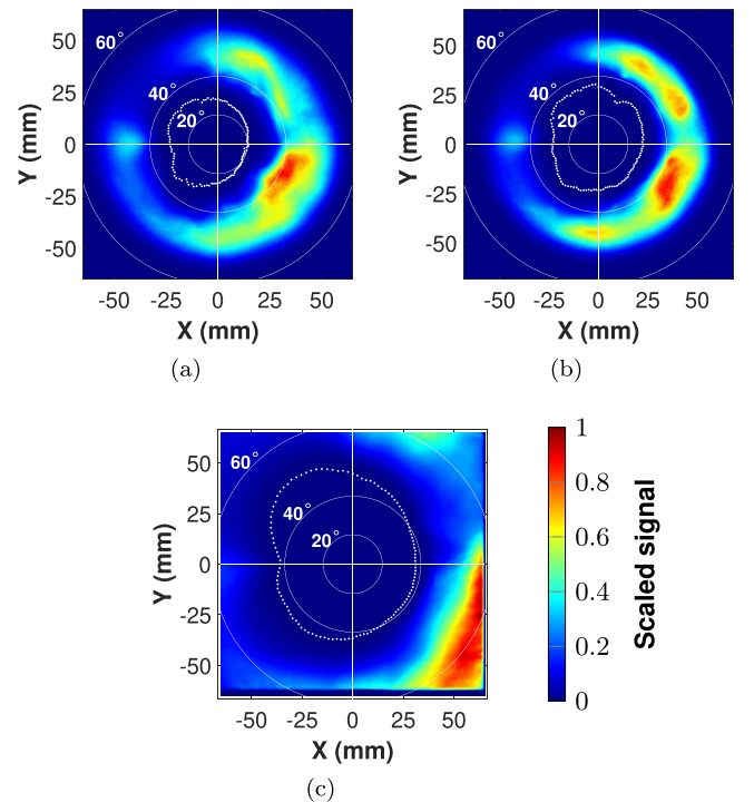
FIG. 2. Scaled image plate data captured under conditions detailed in Table I, where 1 on the color bar corresponds to peak PSL values (see text) of 7.06, 6.82, and 31.88, respectively, for (a)–(c). The laser is polarized along the \vec{x} axis and \vec{k} points into the page. White dots indicate the single-electron PSL level vs \phi (see text).
