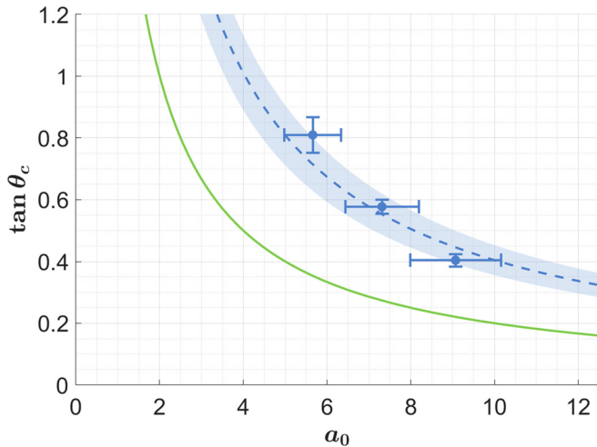
FIG. 6. Energy scaling, \tan \theta_c vs inferred a_0 — 9.1 \pm 1.1 , 7.3 \pm 0.9 and 5.7 \pm 0.7 for the three measurements in Fig. 2 shown by blue filled circles, with Eq. (3) shown by the green solid curve. The inferred a_0 is based on the conditions given in Table I (see Sec. III B). The horizontal error bars, \pm \delta a_0 , represent the uncertainty in calculating a_0 using the low-power focal spot image (Figs. 1(b)–1(d)). The vertical error bars represent the uncertainty in the measurement of \tan \theta_c (see Sec. III A). The blue dashed line represents a numerical fit of the data to \tan \theta_c = 2\eta/a_0 , where \eta = 2.02^{+0.26}_{-0.22} ; the uncertainty in \eta is represented by the shaded region around the dashed curve.
