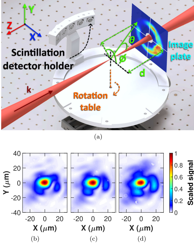
FIG. 1. Experimental setup (not to scale) for image plate and scintillation detectors (a). Image plates are mounted a fixed distance, d \approx 40 mm, after the focus with active area facing the focal spot. Scintillation detectors (not shown) are mounted in the holder, attached to a rotation table, rotating about the focus in the \vec{E}-\vec{k} (i.e., \hat{x}-\hat{z} ) plane a fixed distance ( \approx 138 mm) away. Typical VEGA-3 focal spot images obtained at low power are shown in (b)–(d).
