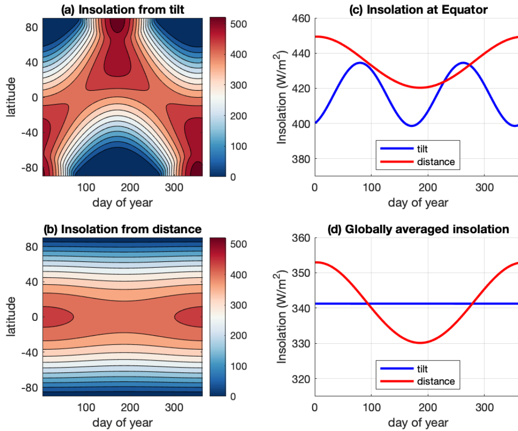
Figure 1. Comparison between the tilt and distance effect on the seasonality of daily-averaged incoming solar radiation (insolation). (a) Insolation resulting from the tilt effect; (b) insolation resulting from the distance effect; (c) insolation at the equator from tilt (blue line) and distance (red line); and (d) globally averaged insolation from tilt (blue line) and distance (red line).
