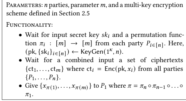
Figure 6: Oblivious Shuffle and Decryption (Shuffle&Decrypt) Ideal Functionality
