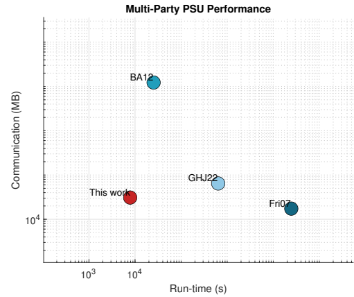
Figure 9: Multi-party PSU protocols with set size of 2^{20} among 4 parties on the network 10Gbps with 0.02ms latency.
