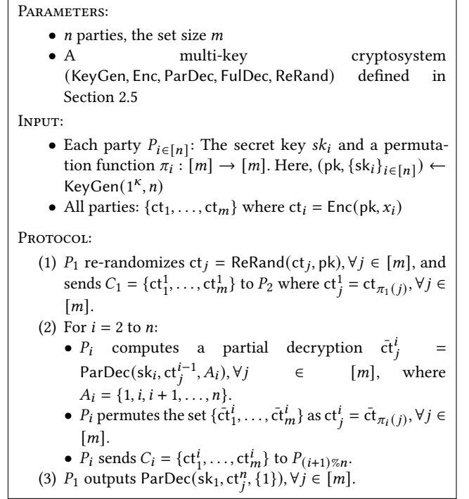
Figure 7: Oblivious Shuffle and Decryption (Shuffle&Decrypt) Construction
