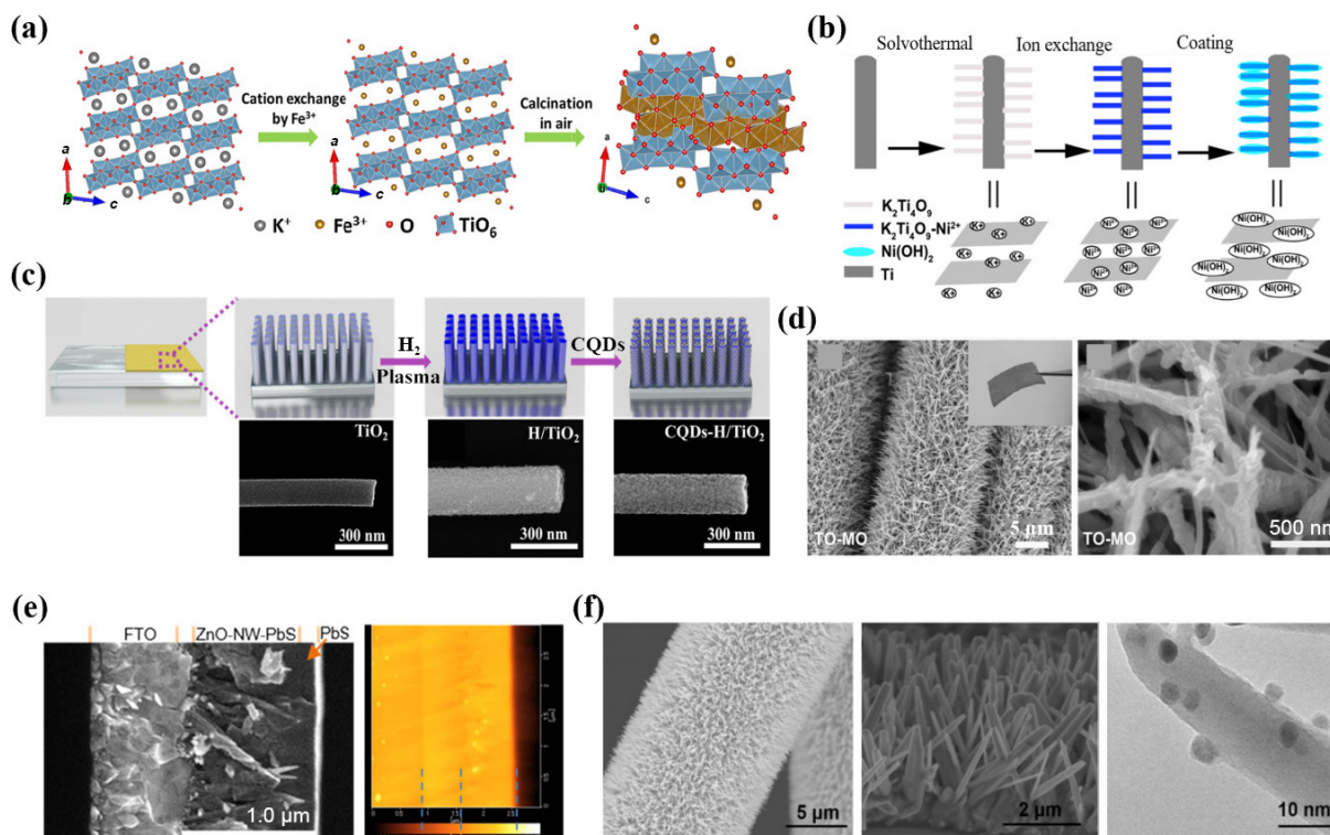
Figure 6 Titanium- and zinc-based nanowires synthesized via solvothermal growth. (a) Schematic illustration of the structures of \text{K}_2\text{Ti}_4\text{O}_9 nanowires, \text{Fe}_2\text{Ti}_4\text{O}_9 nanowires, and \text{Fe-TiO}_x\text{LNWs} (from left to right). Reproduced with permission from Ref. [15], © Elsevier Ltd. 2017. (b) Schematic illustration of the synthesis of \text{Ni(OH)}_2@K_2\text{Ti}_4\text{O}_9 nanowires. Reproduced with permission from Ref. [122], © American Chemical Society 2014. (c) Schematic illustration of the synthesis of \text{CQDs-H/TiO}_2\text{NWs} on FTO glass and corresponding SEM images for each step. Reproduced with permission from Ref. [66], © American Chemical Society 2019. (d) SEM images of \text{MoO}_3 -coated \text{TiO}_2\text{NWs} on carbon cloth. Reproduced with permission from Ref. [123], © WILEY-VCH Verlag GmbH & Co. KGaA, Weinheim 2015. (e) Cross-sectional SEM (left) and AFM (right) images of the \text{PbS QD/ZnONW} -modified solar cell. Reproduced with permission from Ref. [126], © American Chemical Society 2021. (f) SEM images (left and middle) of \text{ZnONWs} on carbon cloth, and TEM image (right) of \text{AgNPs} attached to \text{ZnONWs} . Reproduced with permission from Ref. [68], © Elsevier Ltd. 2017.
