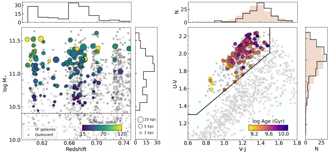
Figure 1. Left: the selected sample in redshift vs. stellar mass space, colored by S/N at rest-frame 5000\text{\AA} . The sizes of each point correspond to the physical half-light radius of the object, with the smallest and largest circles representing 1\text{ kpc} and 10\text{ kpc} , respectively. At higher redshift, fewer quiescent galaxies are included in the sample, as they do not reach the required wavelength range of 5350\text{\AA} . The dashed line shows the 90% mass-completeness limit ( \log M/M_\odot = 10.4 ). Right: the selected sample in UVJ space, colored by best-fit stellar ages from alf . For comparison, both panels show the full LEGA-C data set for the selected redshift range ( 0.6 < z < 0.75 ). The small stars represent star-forming galaxies, and small circles are quiescent, according to their position on the UVJ diagram (Muzzin et al. 2013b). The black histograms show the distribution of the selected sample along each axis. For the UVJ panel, we also include distributions of the quiescent LEGA-C data set in red, normalized to the area of the black histograms.
