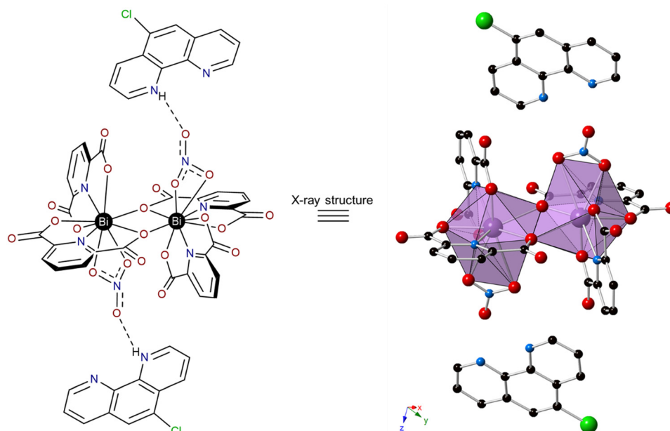
Fig. 5 Left: Illustration of 4. Right: Polyhedral representation of the dimeric unit in 4. Purple = bismuth, blue = nitrogen, red = oxygen, black = carbon, and green = chloride atoms. Hydrogen atoms and lattice water molecules have been omitted for clarity.
