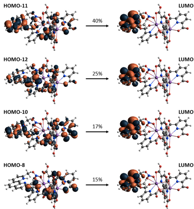
Fig. 13 TD-DFT calculated dominant orbital transitions for the lowest bright excited singlet state of 1 at 330 nm (3.7536 eV) showing BiPDC Bi 6s/PDC \pi and R-Phen \pi donor orbitals with phen \pi^* acceptors.
