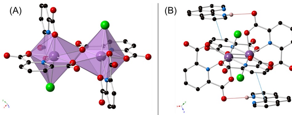
Fig. 6 (A) Polyhedral representation of the \text{BiCl}_2(\text{HPDC})_2(\text{PDC})_2 dimeric unit observed for 5 . (B) Ball and stick model showing the hydrogen bonding interactions (red dashed lines) between PhenH and HPDC, as well as \pi - \pi interactions (blue dashed lines) between PhenH and PDC in 5 . Purple = bismuth, blue = nitrogen, red = oxygen, black = carbon, and green = chloride atoms. Hydrogen atoms and lattice water molecules have been omitted for clarity.
