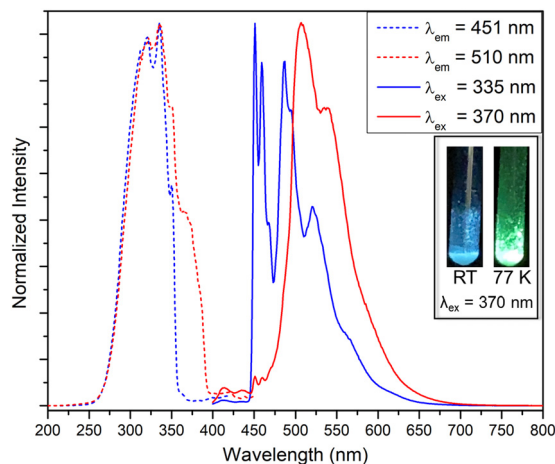
Fig. 8 Low temperature excitation (dashed lines) and emission (solid lines) spectra for compound 2 collected at 77 K. The inset shows the color change of the material upon excitation at 370 nm at room temperature (left) and 77 K (right).
