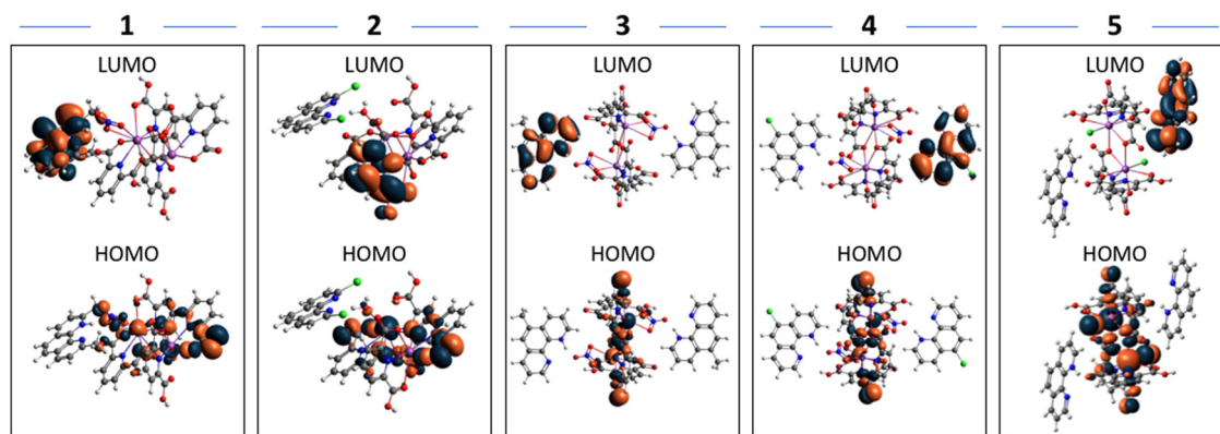
Fig. 12 Isodensity representations of frontier molecular orbitals of 1–5 . The HOMOs consist of BiPDC Bi 6s/PDC \pi orbitals while the R-phen \pi^* comprises the LUMOs.
