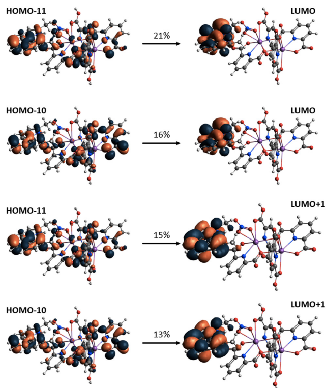
Fig. 14 TD-DFT calculated dominant orbital transitions for the lowest bright excited triplet state of 1 at 431 nm (2.8755 eV).
