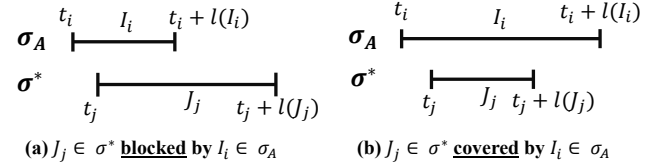
Figure 14: The block and cover relationship between batches in \sigma_{\mathcal{A}} and \sigma_* . Note that if J is identical to I then J is covered by I (by our definition of blocking).
