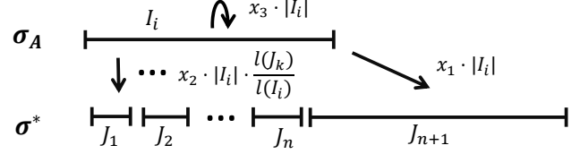
Figure 13: The value assignment rule from one I \in \sigma_{\mathcal{A}} to J_s \in \sigma_* .
