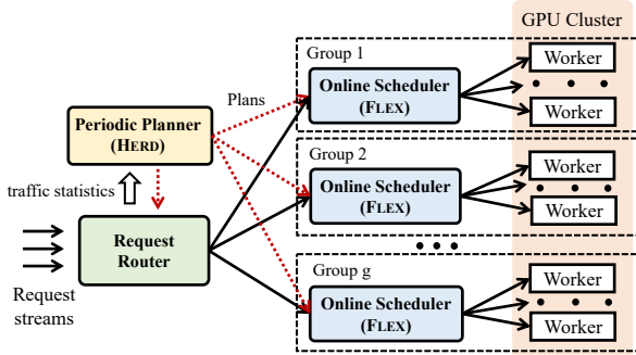
Figure 6: Overview of SHEPHERD design
