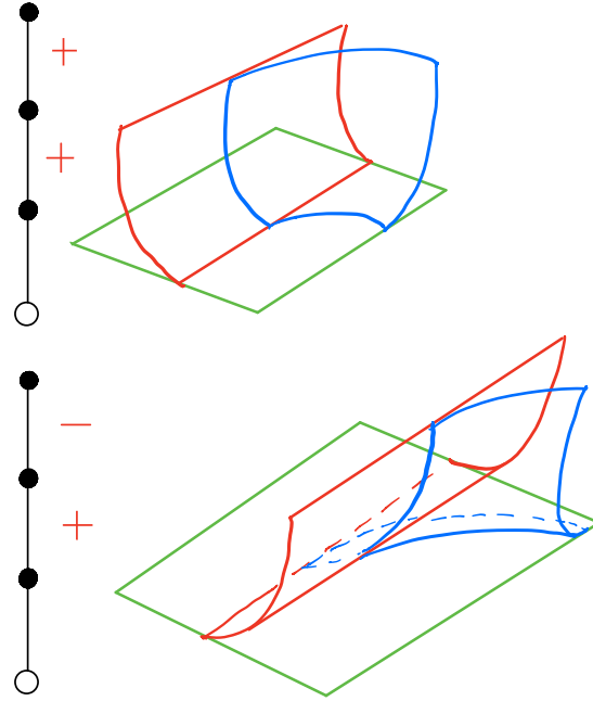
FIGURE 2.5. Two A_4 fronts with different choices of signs. The other two fronts can be obtained from these two by reflections.
