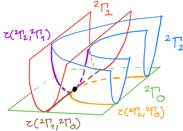
FIGURE 3.4. Verification of the conclusion of Lemma 3.22 for n = 2 , in this case both the right and left hand sides of the equality \tau(\tau({}^2\Gamma_2, {}^2\Gamma_0), \tau({}^2\Gamma_1, {}^2\Gamma_0)) = \tau({}^2\Gamma_2, {}^2\Gamma_1) \cap \tau({}^2\Gamma_1, {}^2\Gamma_0) consist of the origin.
