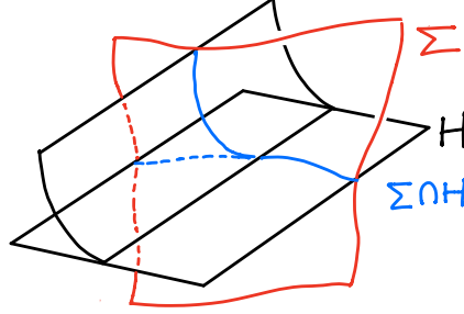
FIGURE 3.3. Illustration that \Sigma \cap H is an arboreal front in \Sigma .
