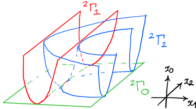
FIGURE 2.2. The hypersurfaces {}^2\Gamma_0 (green), {}^2\Gamma_1 (red) and {}^2\Gamma_2 (blue).
