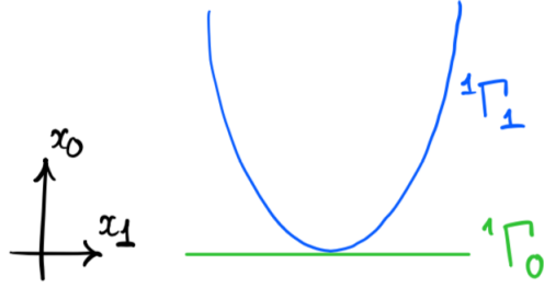
FIGURE 2.1. The hypersurfaces {}^1\Gamma_0 (green) and {}^1\Gamma_1 (blue)
