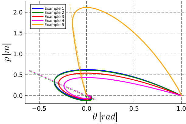
Fig. 3: Simulation results of the closed-loop systems in Examples 1-5 with initial condition (1rad, 0m). The state approaches the origin in all examples except for Example 2, as no feed-forward is used, where the equilibrium is (0rad, -0.02m). Dashed lines indicate the corresponding set F_0 , which overlap for Examples 1, 3 and 4.
