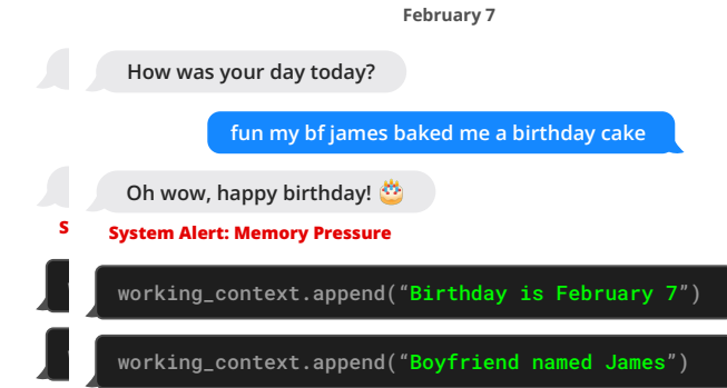
Figure 1. MemGPT can search out-of-context data to bring relevant information into the current context window.
