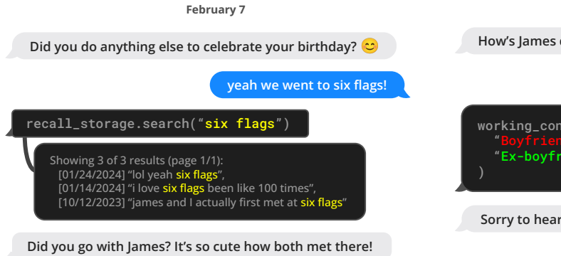
Figure 2. MemGPT (left) can search out-of-context data to bring relevant information into the current context window.
