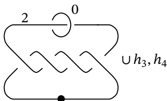
FIGURE 1. Kirby diagram for Z_0 .
