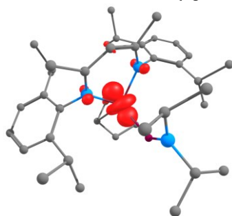
Figure 11. Spin density plot of 6 • . The isosurface value is 0.0518.
