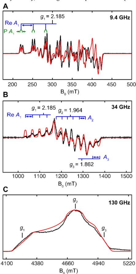
Figure 10. EPR spectra of complex 6 ^\bullet (black traces) and simulations (red traces) at multiple frequencies. (A) X-band CW EPR spectrum of 6 ^\bullet . Acquisition parameters: T = 15 K, fre-
