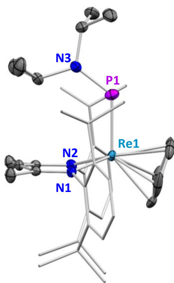
Figure 9. X-ray crystal structure of 6 ^\bullet . The BDI aryl groups are shown in wireframe, hydrogen atoms are omitted for clarity, and ellipsoids are displayed at 50% probability.
