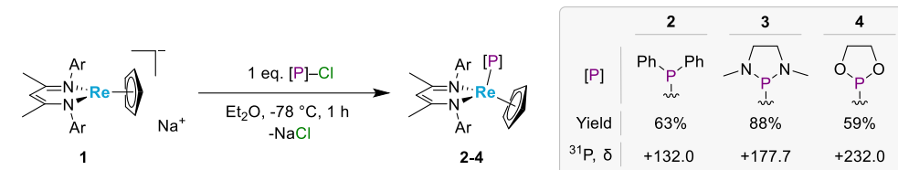
Scheme 1. Synthesis of Phosphido Complexes 2, 3, and 4.
