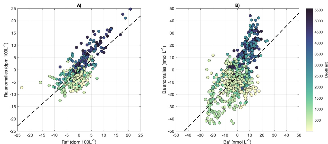
Figure 3. Relationships between Ba* and Ba anomalies along the GP15 section. The color scale represents the depth of each sample. Ba* is calculated from a regression versus Si. The best linear fit ( R^2 = 0.65 , P < 0.0001 ) is also reported (dashed black line). The slope of the Ba* and Ba anomaly relationship is 1.08 \pm 0.03 .
