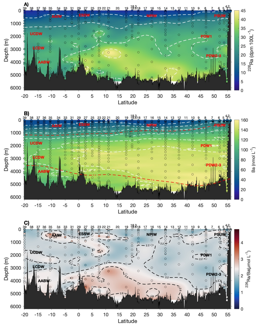
Figure 4. (a) Distribution of dissolved ^{226}\text{Ra} activities ( \text{dpm } 100 \text{ L}^{-1} ), (b) dissolved Ba concentrations ( \text{nmol L}^{-1} ), and (c) dissolved ^{226}\text{Ra}/\text{Ba} ratios along the GP15 section. Station numbers are found on the top of the panel. The sampling depths are shown for each vertical profile (dots). The different water masses are also reported: ESSW: Equatorial Subsurface Water, NPIW: North Pacific Deep Water, PDW: Pacific Deep Water, PSIW: Pacific Subarctic Water, LCDW: Lower Circumpolar Deep Water, UCDW: Circumpolar upper Deep Water, AABW: Antarctic Bottom Water.
