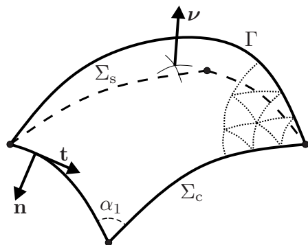
FIG. 1. Illustration of curved surface \Gamma in \mathbb{R}^3 with mesh. The boundary \Sigma \equiv \partial\Gamma decomposes as \Sigma = \Sigma_c \cup \Sigma_s and has a finite number of corners with interior angles \alpha_i . The boundary \Sigma has (outer) conormal vector, \mathbf{n} , and oriented unit tangent vector, \mathbf{t} . The normal vector of \Gamma is \boldsymbol{\nu} . Part of the exact, curved surface triangulation \mathcal{T}_h is shown with dotted curves.
