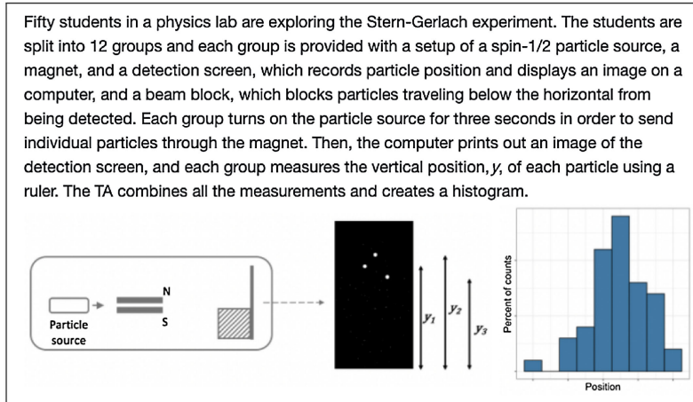
(a) Stern-Gerlach scenario
