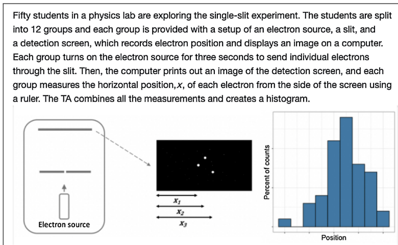
(c) Single slit scenario
