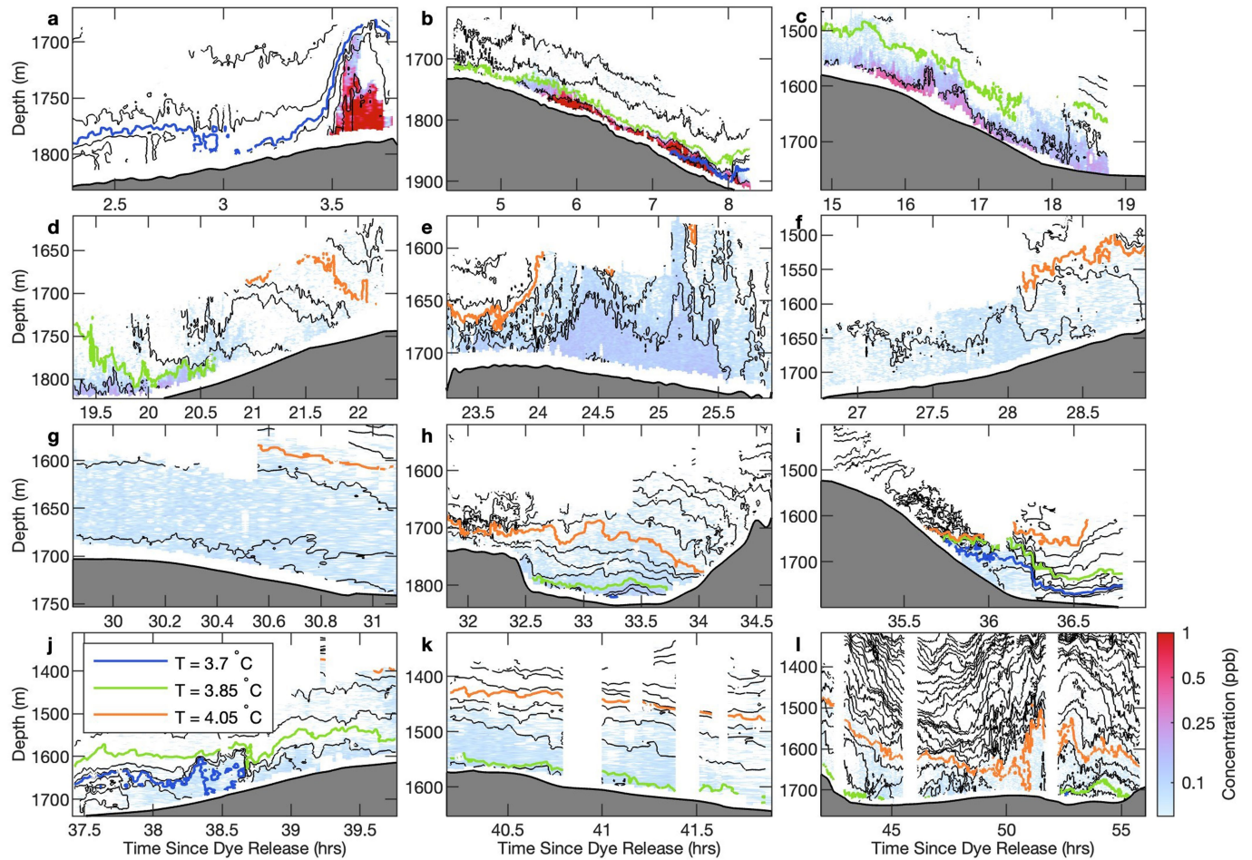
Extended Data Fig. 5 | All transects from the FCTD survey of the dye. (a)-(l) Dye concentration is shown on a logarithmic scale in parts per billion (ppb) in colour, isotherms every 0.05°C are shown with black contours, and
