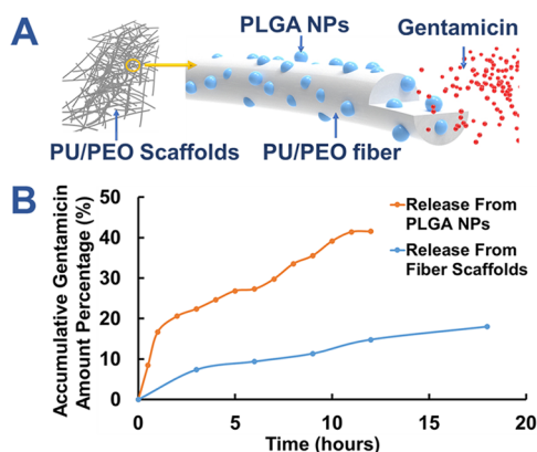
Figure 8. (A) 3D diagram showed gentamicin release from the PLGA nanoparticle-incorporated fibers. (B) Release profile of fibers. Accumulative gentamicin amount percentage released from NPs and fibers scaffolds at different times.
