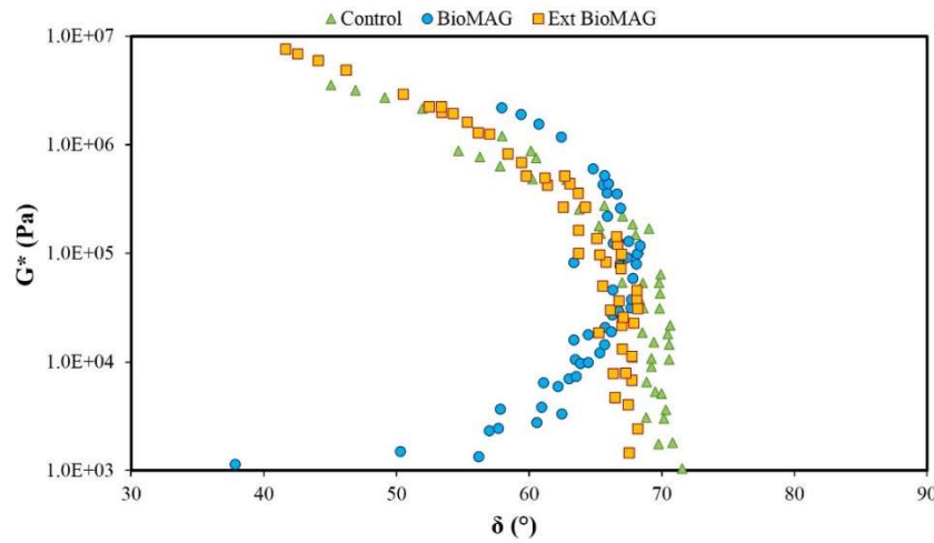
Fig. 4. Black space diagram of the control, BioMAG and extracted BioMAG asphalt binders.
