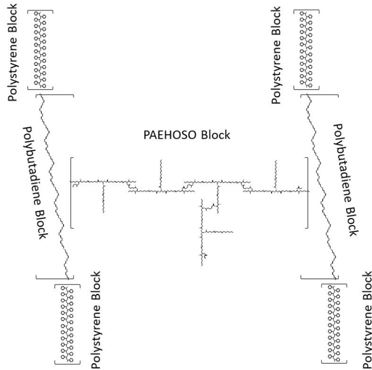
Fig. 1. Schematic of the reaction mechanism of PAEHOSO with the butadiene group of SBS.
