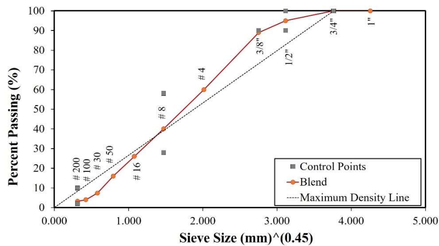
Fig. 2. Gradation of aggregate blend.
