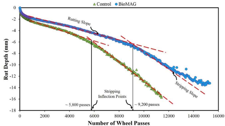
Fig. 7. Sample HWT test data plotted and analyzed for two mixture groups.
