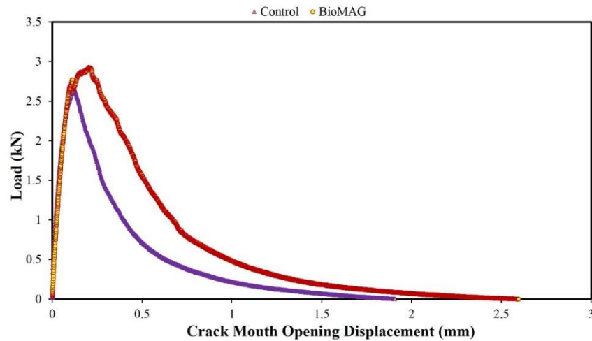
Fig. 6. Sample DCT test data plotted for two mixture groups.
