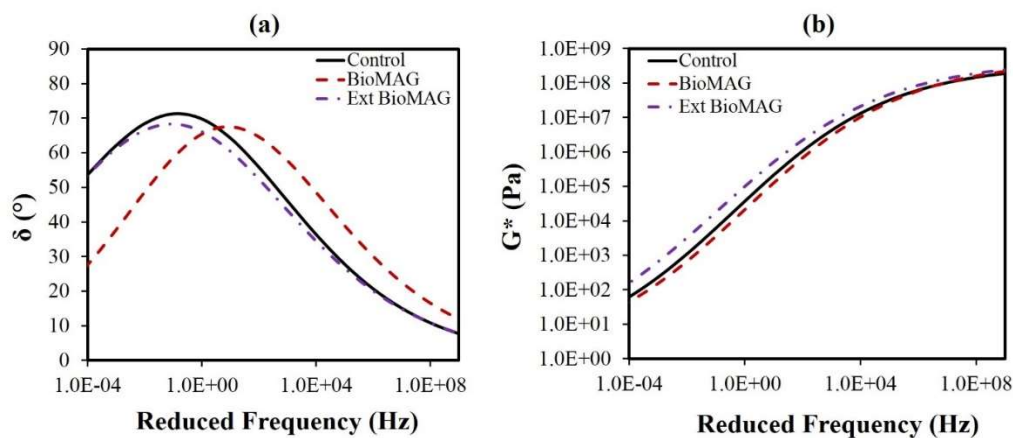
Fig. 3. Phase angle (a) and complex shear modulus (b) master curves constructed for asphalt binders at a reference temperature of 34°C.
