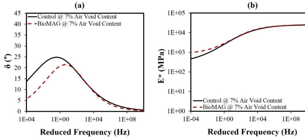
Fig. 5. Phase angle (a) and dynamic modulus (b) master curves constructed for asphalt mixtures at a reference temperature of 21°C.
