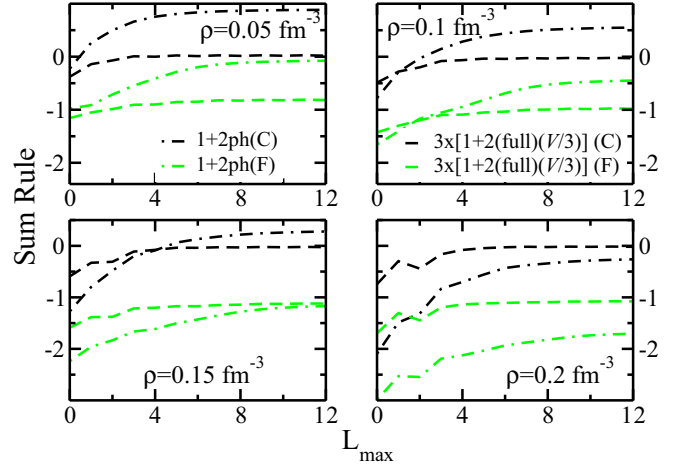
FIG. 3. Same as Fig. 3, but for cases “1+2(ph)” (dash-dotted) and “ 3 \times [1+2(\text{full}) (V/3)] ” (dashed lines). See text for details.
