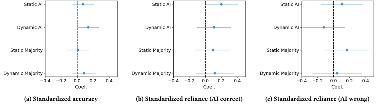
Figure 3: Estimated coefficients from linear regression models for predicting a group’s (a) standardized accuracy, (b) standardized reliance on correct AI recommendations, and (c) standardized reliance on incorrect AI recommendations. The error bars indicate the 95% confidence intervals. For standardized accuracy and standardized reliance on correct AI recommendations, an interval above zero is better; for standardized reliance on incorrect AI recommendations, an interval below zero is better.
