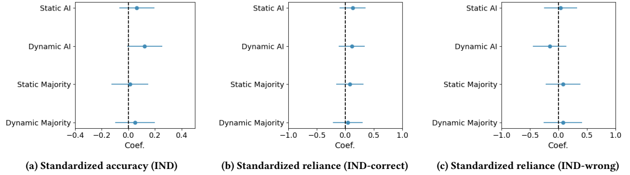
Figure 4: Estimated coefficients from linear regression models for predicting a group’s (a) standardized accuracy on all in-distribution tasks, (b) standardized reliance on in-distribution tasks where the AI recommendation is correct, and (c) standardized reliance on in-distribution tasks where the AI recommendation is wrong. The error bars indicate the 95% confidence intervals. For standardized accuracy and standardized reliance on correct AI recommendations, an interval above zero is better; for standardized reliance on incorrect AI recommendations, an interval below zero is better.
