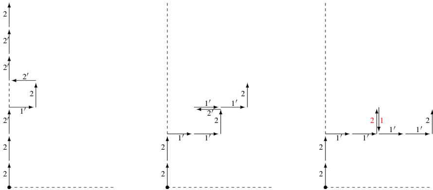
Fig. 7 From left to right, the walks of T^+ , E_1^{k-1}(T^+) , and E'_1 \circ E_1^{k-1}(T^+) , where T is a tableau with reading word 111'\Box 11'1'1'1 . The special entries, t and u , are red and in boldface
