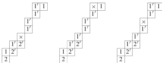
Fig. 9 The elements, in order, of an \omega_{i'} = \text{sh}_{1'} \circ \text{esh}_{1'} orbit
