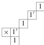
Fig. 8 A shape and content giving rise to a Schubert curve S with many complex components
