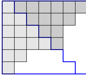
Fig. 2 A strict partition \sigma = (6, 4, 2, 1) shown above the diagonal. Its associated symmetric partition \tilde{\sigma} = (7, 6, 5, 5, 2, 1) is the union of the two shaded regions shown
