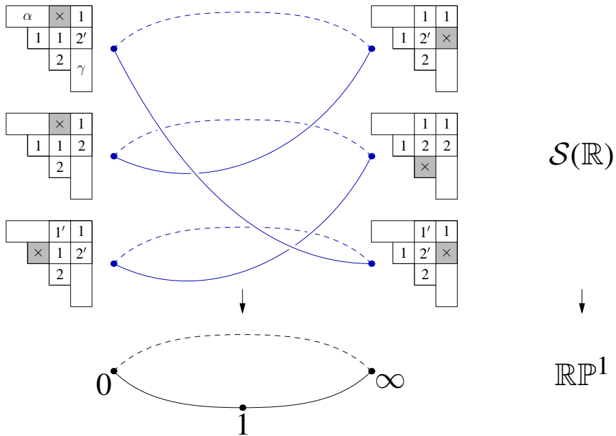
Fig. 1 The covering map S(\mathbb{R}) \rightarrow \mathbb{RP}^1 , along with the canonical labeling of the fibers over 0 and \infty
