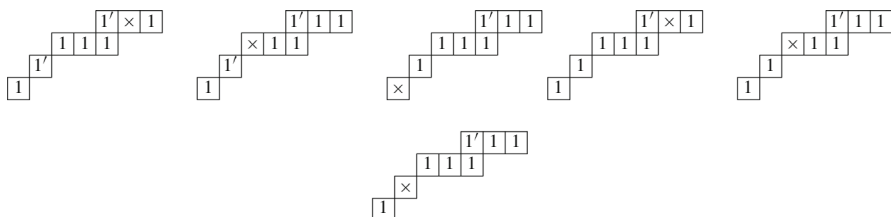
Fig. 10 An \text{sh}_1 \circ \text{esh}_1 -orbit involving an exceptional move. The exceptional move occurs on the step from the last element to the first element shown above
