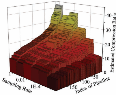
Fig. 12. Estimated Compression Ratios with Different Sampling Rates
