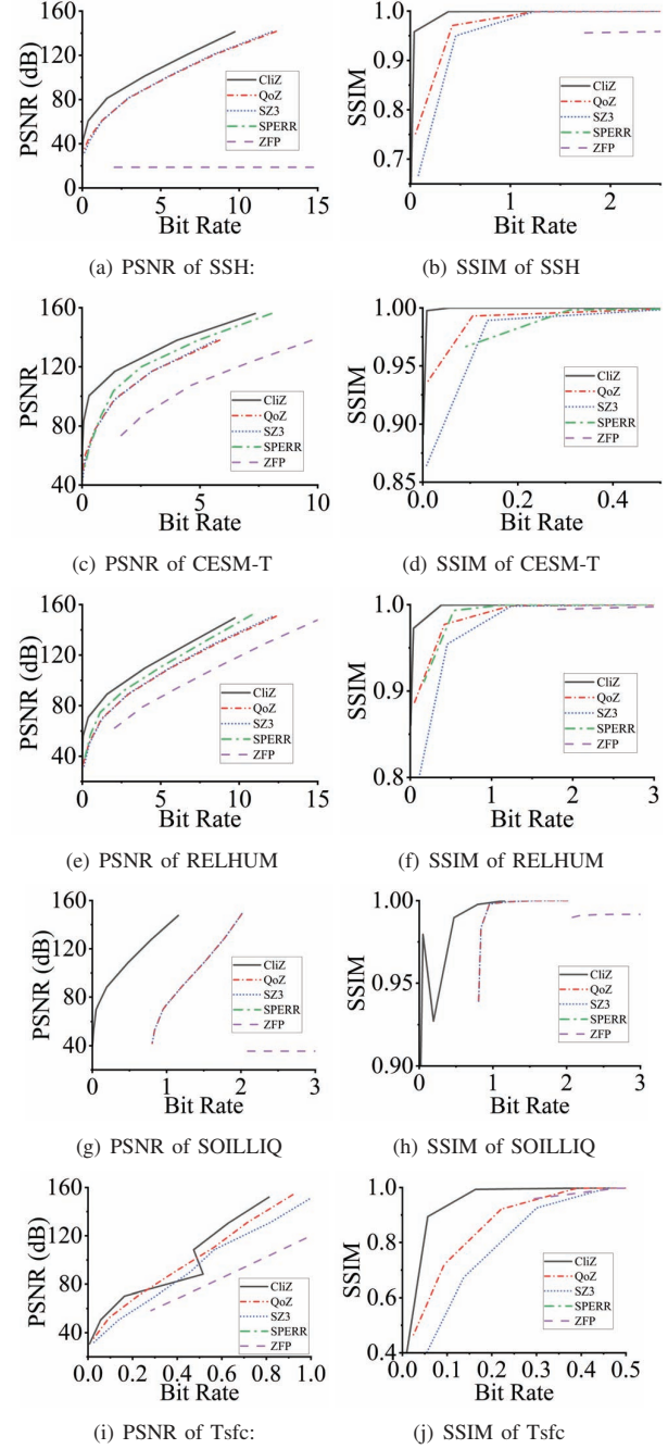
Fig. 10. Rate-distortion graphs
