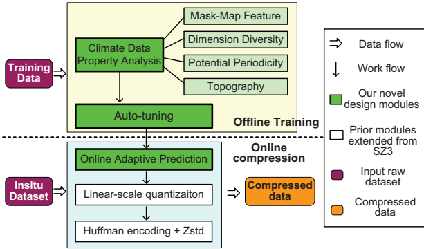
Fig. 1. Design Overview of CliZ
