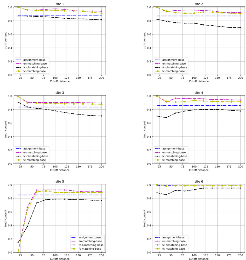
Figure 5. Precision of conflation models for the Santa Barbara road networks (OSM vs. TIGER).
