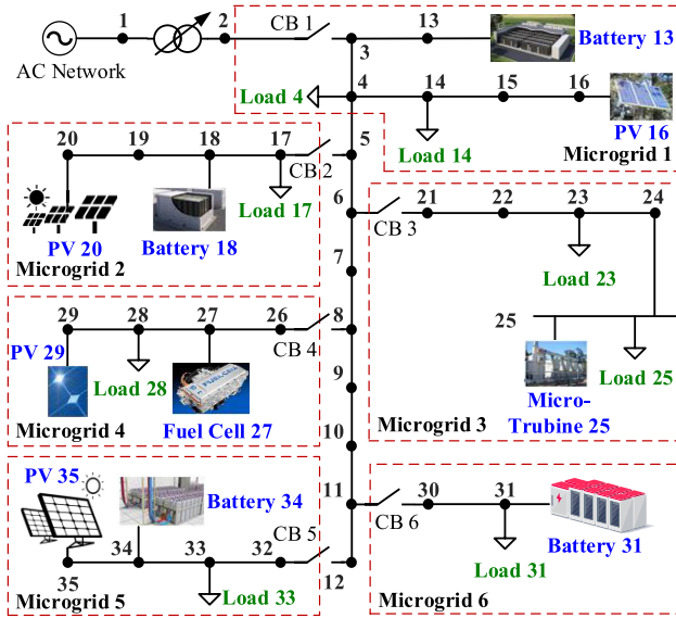
FIGURE 2. Networked microgrid test system.
