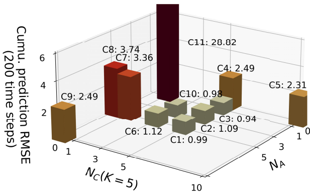
FIGURE 6. Impact of processor layers on the model performance.
