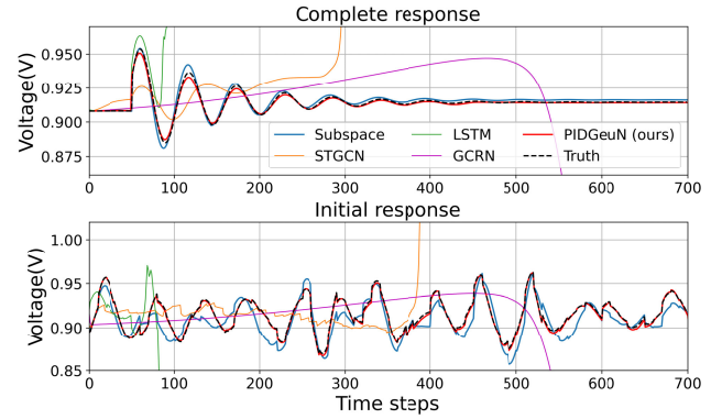
FIGURE 3. Complete and initial voltage dynamic response of a DER bus.
