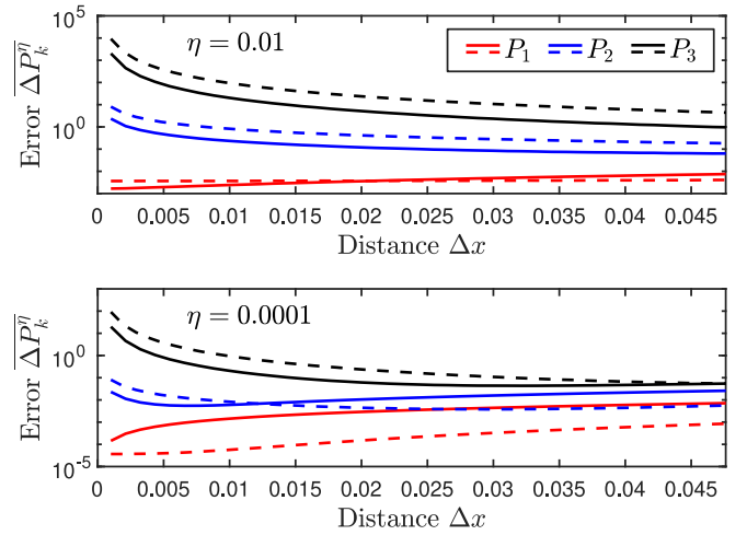
FIG. 7. Comparison of time-averaged error \overline{\Delta P_k^\eta} [Eq. (30)] for accuracy a = 1 (solid curves) and a = 2 (dashed curves). The used parameters are identical to those used for Fig. 5. Shown are the time-averaged errors for P_1 (red), P_2 (blue), and P_3 (black curves), for noise amplitude \eta = 10^{-2} (upper panel) and \eta = 10^{-4} (lower panel).
