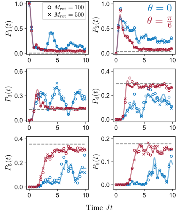
FIG. 6. Application of Method B to obtaining the operator size distribution \{P_k(t)\} for the case of the Ising model of Eq. (23) with N = 6 and J/B = 1 . Each panel shows a different value of k = 1, \dots, 6 . Full lines correspond exact numerical results obtained by solving the Heisenberg evolution of the initial operator, here chosen to be W(0) = \sigma_x^{(1)} . Symbols correspond to numerical simulations of Method B (Sec. IV) with different choices of the number of sampled rotations M_{\text{rot}} = 100 (circles) and M_{\text{rot}} = 500 (crosses). Different colors denote different regimes of the model: integrable case \theta = 0 (blue) and chaotic case ( \theta = \pi/6 ) (red).
