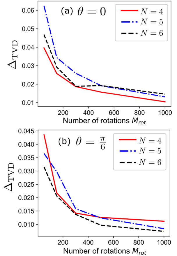
FIG. 9. Time-averaged total variational distance, defined in Eq. (C4), between the exact operator size distribution \{P_k(t)\} and the approximate one obtained by Method B \{\tilde{P}_k\} , as a function of the number of rotations used by the method, M_{\text{rot}} . Panel (a) shows results for the integrable Ising model \theta = 0 , while (b) corresponds to the chaotic case \theta = \pi/6 . We observe that the error in reconstructing the full probability distribution decays with M_{\text{rot}} , with no strong dependence on system size N . General evolution parameters are the same as used in Fig. 6.
