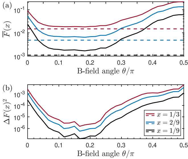
FIG. 4. (a) Time average \bar{F}(x) and (b) fluctuations \Delta F(x)^2 of the PGF F(x, t) as a function of the B-field angle \theta , plotted for three values of x corresponding to \varepsilon = 1 (red), \varepsilon = \sqrt{2/3} (blue), and \varepsilon = \sqrt{1/3} (black curve). The time average and fluctuations are calculated for 5 \leq Jt \leq 80 to exclude the initial transient dynamics from the results. In (a) we compare the time average \bar{F}(x) (solid lines) with the PGF value for a Haar-random probability distribution (dashed lines).
