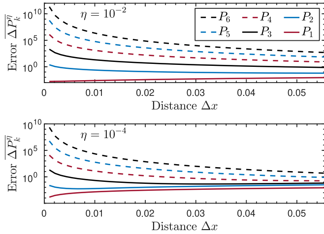
FIG. 5. Time-averaged error \overline{\Delta P_k^\eta} [see Eq. (30)] for the elements of the probability distribution \{P_k\} , averaged over 0 \leq Jt \leq 10 . We have used multiplicative noise with strength \eta = 10^{-2} (upper panel) and \eta = 10^{-4} (lower panel), added to the PGF F(x, t) before using finite-difference derivatives with step size \Delta x and accuracy a = 2 to extract the noisy probability distribution elements \{P_k^\eta(t)\} . In both panels the curves from top to bottom at \Delta x = 0.02 are the time-averaged errors \overline{\Delta P_k^\eta} for P_6 (black dashed), P_5 (blue dashed), P_4 (red dashed), P_3 (black solid), P_2 (blue solid), and P_1 (red solid), averaged over 100 noise realizations.
