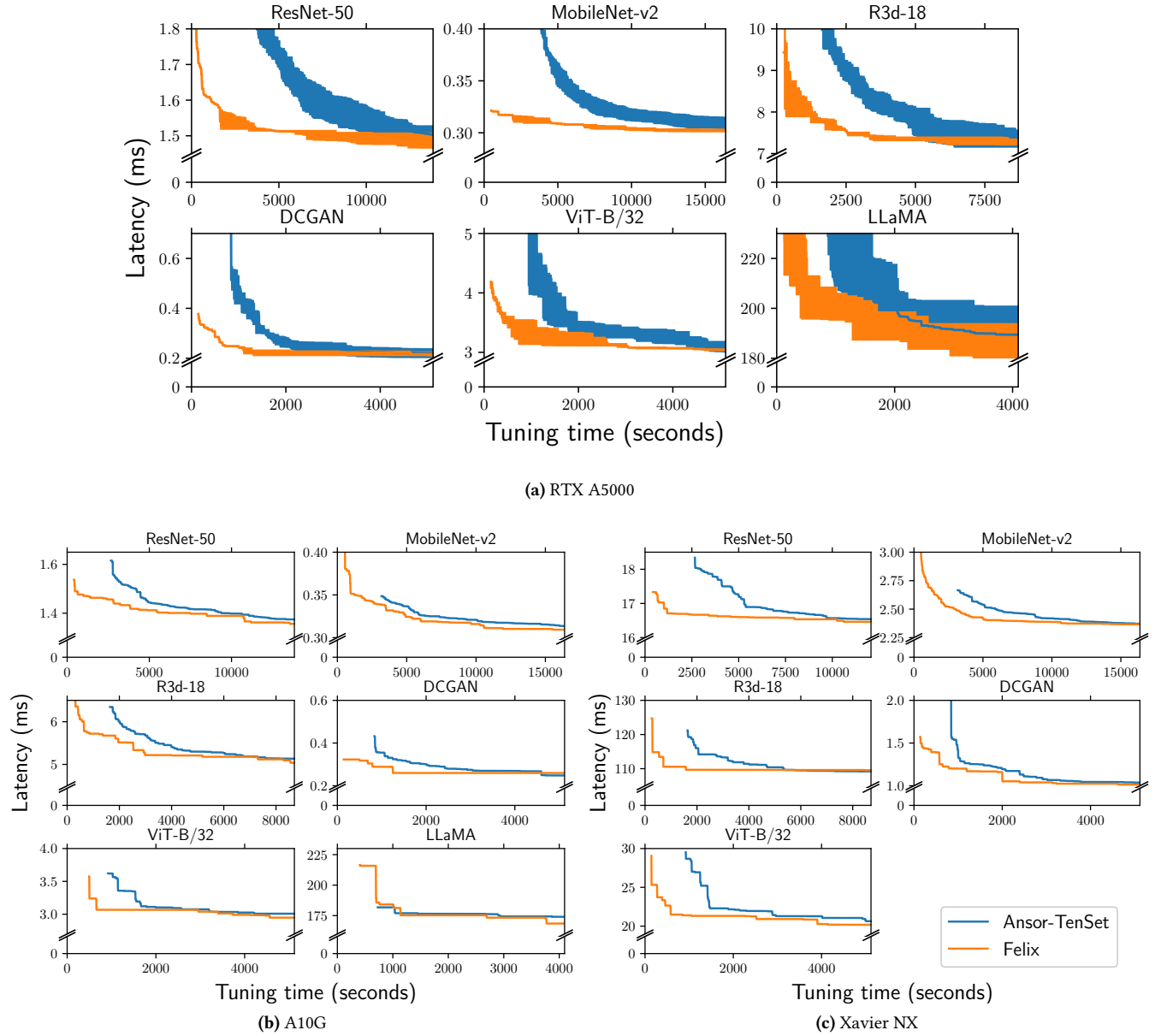
Figure 7. Best performance (shown as network inference latency) vs. search time during the schedule search of Felix and Ansor-TenSet.
