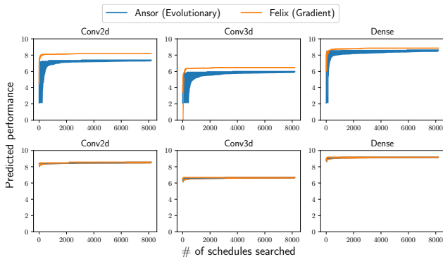
Figure 8. Predicted performance of the candidate schedule population as the search progresses in Felix and Ansor. The top row shows earlier tuning iterations close to the beginning of the tuning session. and the bottom row shows later tuning iterations close to convergence (both tools' lines overlap).
