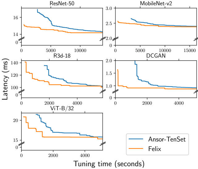
Figure 10. Best performance (network inference latency) vs. search time during the schedule search of Felix and Ansor-TenSet. The networks are optimized for RTX A5000 with a input batch size of 16.
