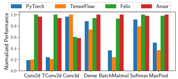
Figure 9. Single operator performance of Felix, Ansor, and manually-optimized libraries (PyTorch, TensorFlow) on RTX A5000. The y-axis is the performance of one framework normalized to the best performance across all frameworks for an operator.
