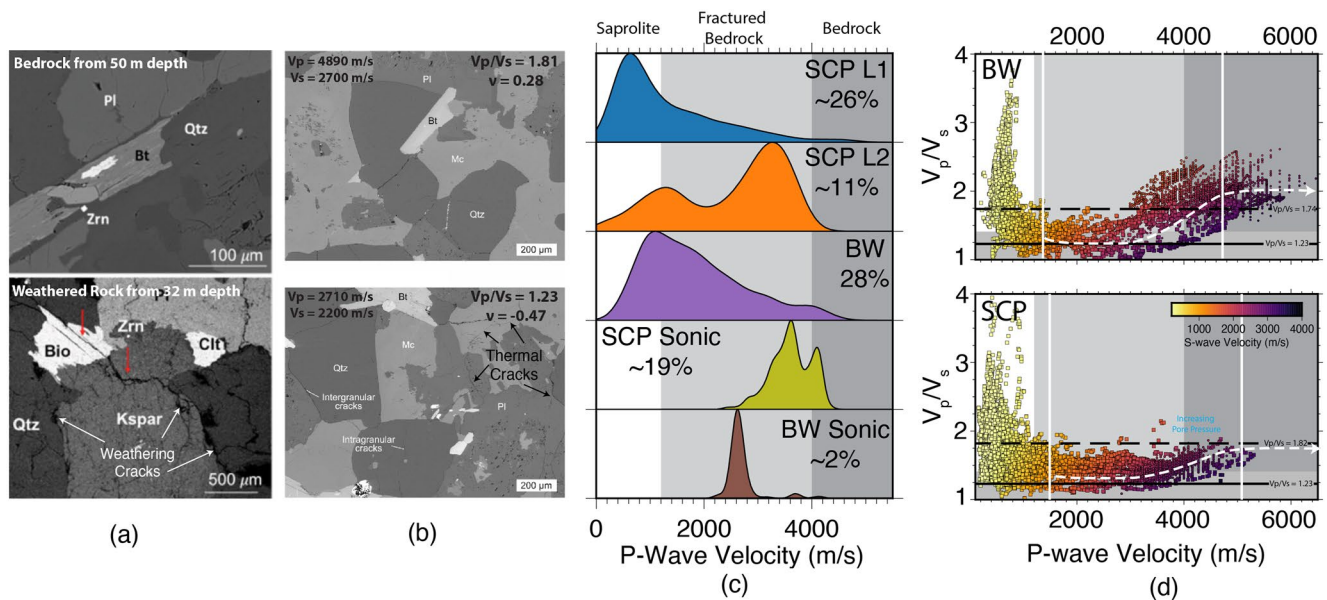
Figure 4. (a) SEM sections from a borehole \sim 3 km Southwest of our location (Holbrook et al., 2019). The top panel shows an unweathered bedrock sample from 50 m depth and the bottom shows a weathered bedrock from 32 m depth. (b) SEM sections from a thermally treated granite from Griffiths et al. (2018). The top is the untreated sample, and the bottom plot is an SEM section after being heat treated to 450 C to induce microcracks. The samples' V_p , V_s , V_p/V_s values, and Poisson's ratios are reported on the panels. (c) Probability density functions of V_p for all data with V_p/V_s values less than 1.4 ( \nu < 0 ). The percentage data with values less than 1.4 are shown in each plot. Background colors are CZ structure based on V_p . White is sapolite ( V_p \leq 1,200 m/s), gray is fractured bedrock ( 1,200 m/s < V_p \leq 4,000 m/s), and dark gray is unfractured bedrock ( V_p > 4,000 m/s). (d) V_p/V_s values plotted as a function of V_p and colored by V_s . Gray shaded regions are the same as panel d with an additional gray rectangle to highlight V_p/V_s values less than 1.4. The top panel is for BW. The bottom panel is for SCP, which includes both SCP L1 and SCP L2. Squares are data from seismic refraction surveys, and circles are from sonic logs. The dashed black line is the theoretical V_p/V_s values assuming no porosity based on the mineralogic compositions from Flinchum et al. (2018a) and Flinchum et al. (2018b) for BW and Holbrook et al. (2019) for SCP (Supporting Information S1). The solid black line is the V_p/V_s value from the thermally treated granite shown in panel c. The dashed white line is our interpretation of the V_p/V_s value behavior as physical and chemical weathering creates porosity. The vertical white lines are approximate boundaries of change. The line at the highest P-wave velocities marks the onset of weathering, and the line around 1,200 m/s marks the location where V_p/V_s values increase.
