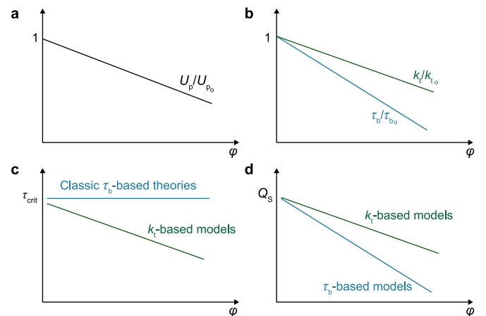
Fig. 4. A schematic diagram showing the impacts of emergent vegetation on the surface flow and bedload transport under the same water surface or energy slope within a vegetation patch. The subscript “o” denotes the value for cases without vegetation, or \phi = 0 . a. At the same water surface slope, U_p decreases with increasing \phi . b. Due to the vegetation-generated additional turbulence, with increasing vegetation volume fraction \phi , the turbulent kinetic energy k_t decreases much slower than the bed shear stress \tau_b . c. The classic \tau_b -based models overestimate the critical shear stress \tau_{\text{crit}} . d. The classic \tau_b -based models underestimate the bedload transport rate Q_s . Note that the lines in the figure show the general tendency instead of the actual relationship, which is not linear.
