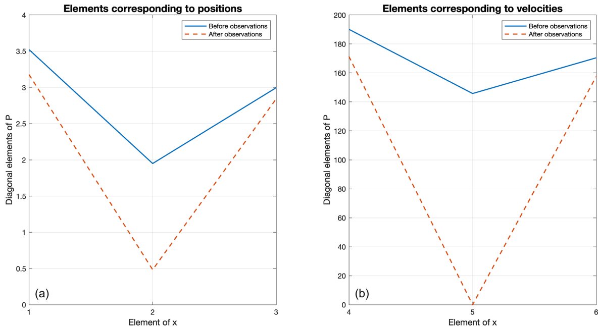
Figure 8. From left to right: (a) the first three diagonal elements of \mathbf{P} before any observations of x_5 (solid) and after 10 observations of x_5 (dashed). (b) The last three diagonal elements of \mathbf{P} before any observations (solid) and after 10 observations (dashed.)
