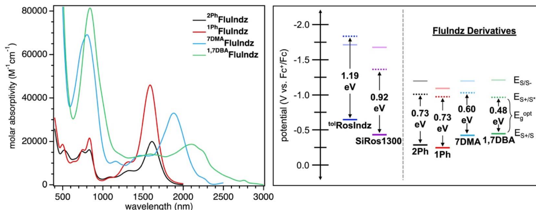
Fig. 2 Molar absorptivity of FluIndz dyes in \text{CS}_2 (left) and electrochemical potentials ( E_{\text{S}+/ \text{S}} , E_{\text{S} / \text{S}^-} , and E_{\text{S}+/ \text{S}^*} ) with optical energy gaps in DCM (right). Electrochemical potentials shown are referenced to \text{Fc}^+/\text{Fc} at 0.00 V in DCM with a 0.1 M \text{Bu}_4\text{NPF}_6 supporting electrolyte.
