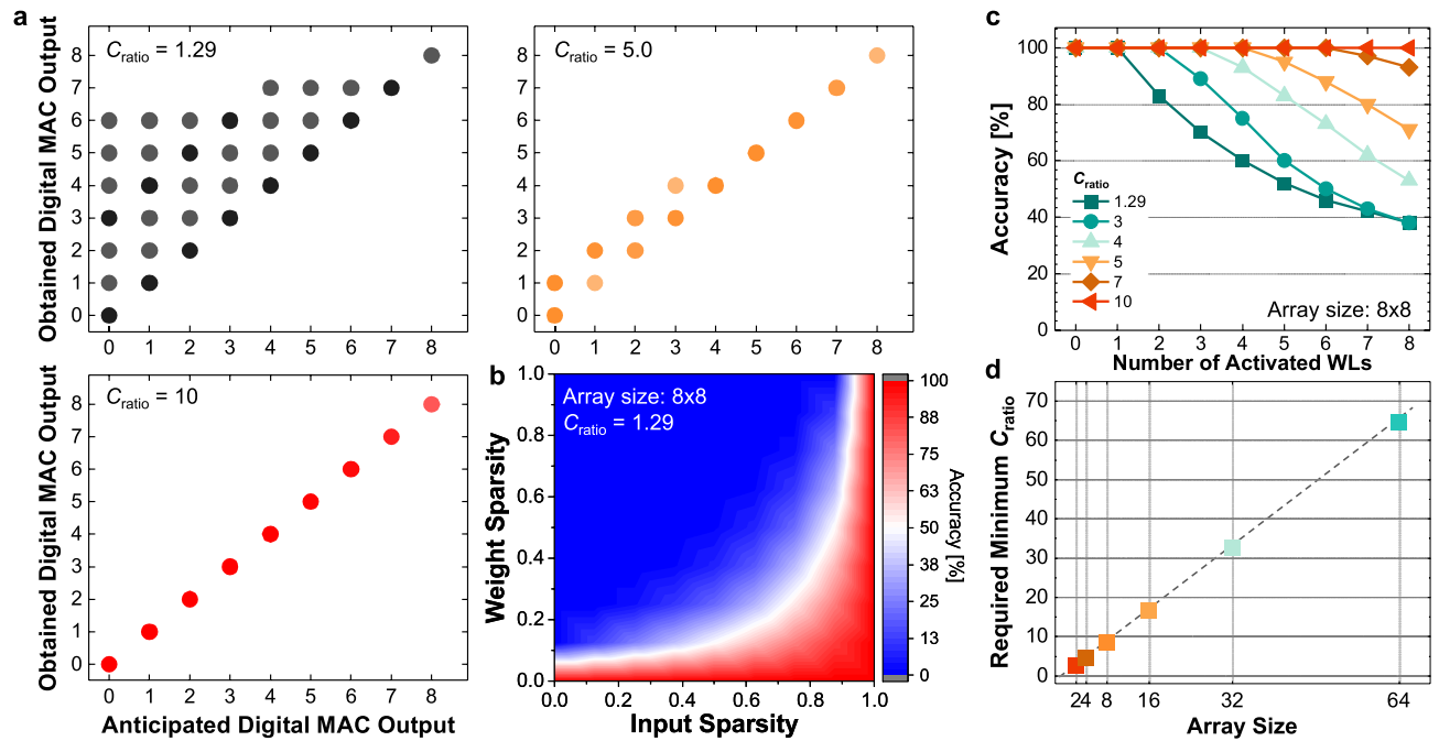
Figure 6. 8 × 8 size FeCap crossbar array, operation schemes, and its performance. (a) Comparison of anticipated digital MAC output with obtained digital output from FeCap-based crossbars at C_{ratio} = 1.29 , 5.0, and 10. Cases with low C_{ratio} exhibit considerable error in obtained MAC output originated from leakages during the activation of LCS. (b) Heatmap of accuracy with respect to input and weight sparsities at 1.29 of C_{ratio} . (c) Accuracy of MAC output for different C_{ratio} and increasing number of activated WLs. (d) Minimum value of C_{ratio} required for varying FeCap-based crossbar array sizes.
