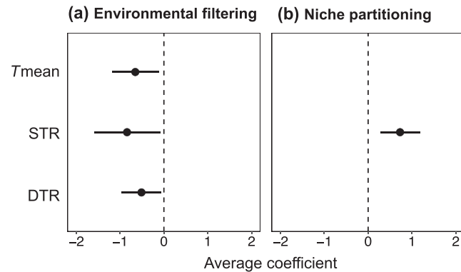
FIGURE 5 Effects of the annual mean temperature ( T_{\text{mean}} ), seasonal temperature range (STR) and diurnal temperature range (DTR) on the strength of environmental filtering and niche partitioning in shaping the body size composition of the 13 moth assemblages. The dots and lines represent the model-averaged coefficients for the variables and their 95% confidence intervals, respectively, in the linear regression models for the strength of environmental filtering (a) and niche partitioning (b). The strength of the two processes was measured by SES_{IC/IR} and SES_{IP/IC} respectively. The values are shown only for the variables included in the final models.
