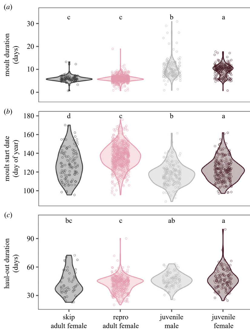
Figure 4. Violin plots and individual values (dots) of moult duration (a), moult start date (b) and haul-out duration (c) for four age-sex categories. Moults are significantly shorter in adult females and later in reproductive adult females as compared with juveniles of both sexes, despite relatively similar haul-out durations. Two or more predictors with the same grouping letter were not different at the \alpha = 0.05 level.
