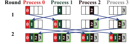
Fig. 3: Recursive doubling for allgather with 4 processes.
