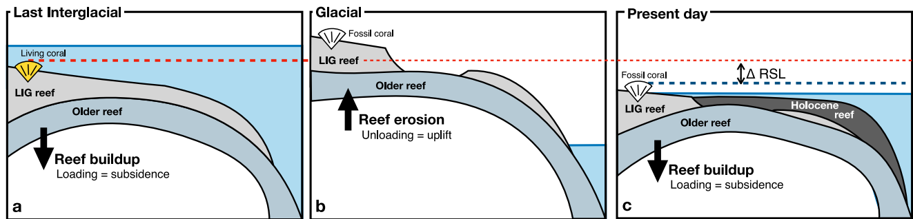
Fig. 3 Illustration of reef isostasy caused by the buildup of the reef complex since the Last Interglacial. a The LIG reef is built on top of an older reef (or the bedrock). The addition of this load leads to isostatic subsidence of the underlying bedrock. b As GMSL falls (e.g., under glacial conditions), the reef is partially eroded and/or dissolved (e.g., by karst processes), resulting in isostatic rebound. c As sea level rises a second time, the reef starts to build again on top of previous structures, causing additional subsidence. \Delta RSL represents the relative sea-level change caused by reef isostasy. The colored dashed lines represent the elevation of the coral during the LIG (red) and its present-day elevation (blue). Note that the uplift and subsidence following reef loading and unloading are transient through glacial-interglacial times, and that in our study we do not model the uplift following reef erosion, which we consider to be balanced with Holocene re-growth.
