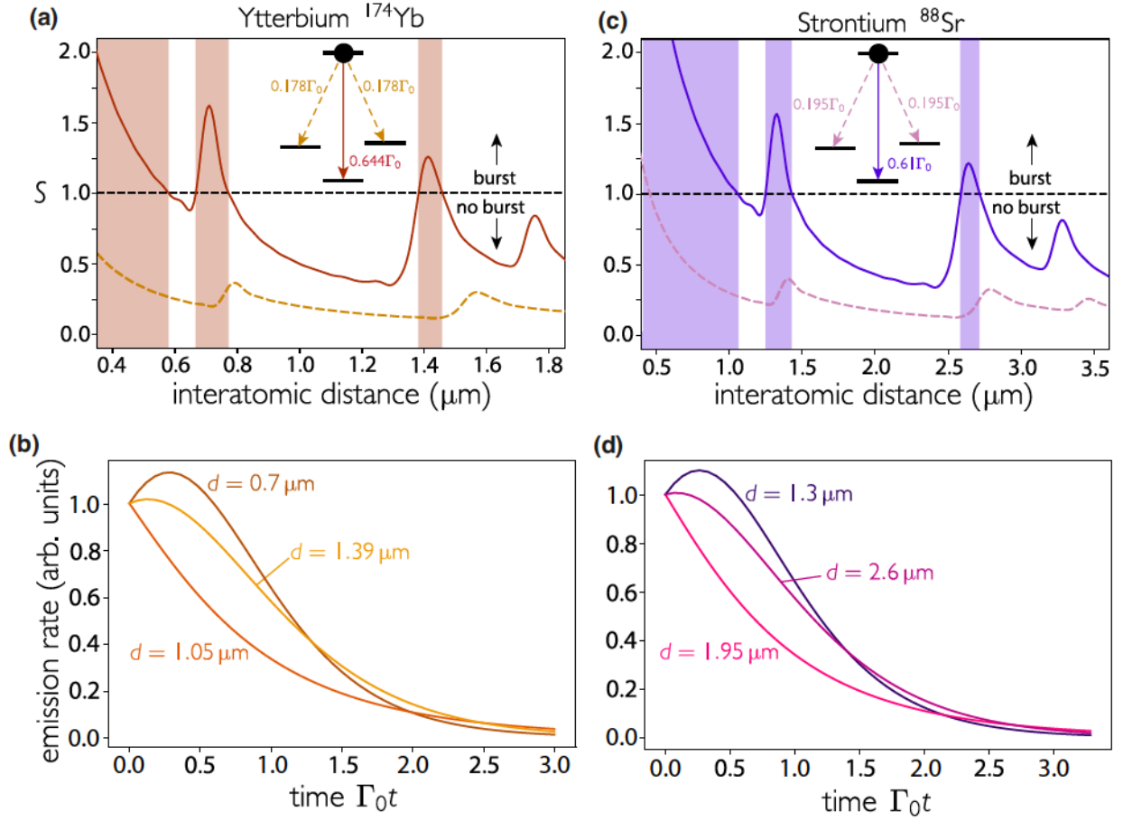
FIG. 5. Predictions of a burst versus lattice constant in 12 \times 12 arrays of (a),(b) ^{174}\text{Yb} and (c),(d) ^{88}\text{Sr} . The atoms are prepared in the ^3D_1 |J=1, m_J=0\rangle state initially and allowed to decay, with the linear transition polarized perpendicular to the array. Light is detected along the x axis. (a),(c) The shaded areas indicate a burst on the ^3D_1 |J=1, m_J=0\rangle \rightarrow ^3P_0 |J=0, m_J=0\rangle transition (red line), as the quantity S in Eq. (18) is larger than 1 (black dashed line). (b),(d) Approximations of the full dynamics via a second-order cumulant expansion (on the ^3D_1 \rightarrow ^3P_0 transition) at three particular distances. As predicted by the superradiance condition, as the distance increases, the superradiant burst disappears and then reappears.
