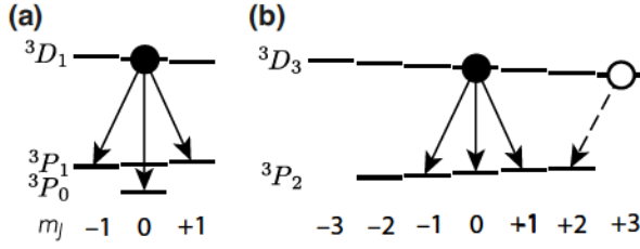
FIG. 4. The considered level structures. Atoms are initialized in the (a) ^3D_1 |J=1, m_J=0\rangle or (b) ^3D_3 |J=3, m_J=0, 3\rangle state. In both m_J=0 cases, the internal structure is simplified into a toy model with three decay channels: a dominant linear \pi -polarized channel and two circularly polarized channels. In (a), the ^3P_1 |J=1, m_J=0\rangle state is not considered, as the transition is forbidden.
