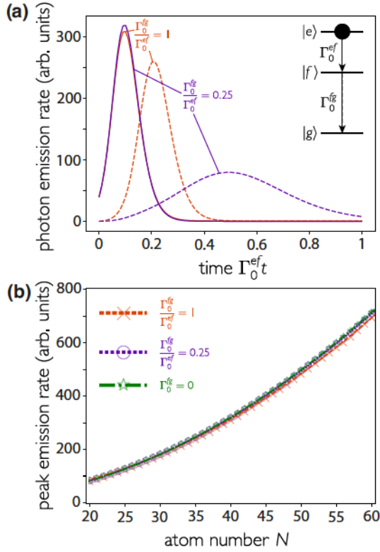
FIG. 3. Superradiant decay from ladder atoms at a point. Each atom decays initially at a rate \Gamma_0^{\text{eff}} to an intermediate state that itself decays at a rate \Gamma_0^{\text{fg}} . (a) Superradiant bursts emitted by 40 ladder atoms. The solid (dashed) lines indicate emission on the initial (secondary) transition. (b) The scaling of the peak emission by N ladder atoms. The lines are power-law best fits of data from N \geq 20 . In all three cases, the fit scales as \sim N^2 .
