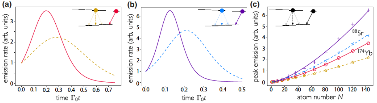
FIG. 7. The largest superradiant burst in ordered 2D arrays of AEs. (a) ^{174}\text{Yb} and (b) ^{88}\text{Sr} atoms are initialized in ^3D_3 |J=3, m_J=0\rangle , with the dominant linear transition polarized perpendicular to the array, or ^3D_3 |J=3, m_J=3\rangle , with the only possible decay having \sqrt{1/2}(\hat{y} + i\hat{z}) polarization. Second-order cumulant-expansion simulations of the superradiant burst emitted on the (dashed) ^3D_3 |J=3, m_J=0\rangle \rightarrow ^3P_2 |J=2, m_J=0\rangle , with parasitic decays to |J=2, m_J=\pm 1\rangle , and (solid) ^3D_3 |J=3, m_J=3\rangle \rightarrow ^3P_2 |J=2, m_J=2\rangle transition. (c) The scaling of the peak emission rate with the atom number. The lines are power-law fits of data with N \geq 25 . For the two-level system, the scaling of the peak is N^{1.38} for ^{174}\text{Yb} and N^{1.47} for ^{88}\text{Sr} , while the four-level system scales as N^{1.29} for ^{174}\text{Yb} and N^{1.37} for ^{88}\text{Sr} . In all plots, the lattice constant is d = 244 nm.
