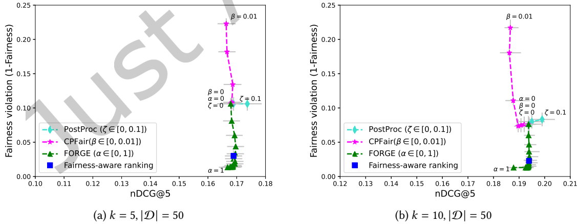
Fig. 8. MovieLens1M data with VAE CF as base-ranker— average nDCG vs. average 1 - \text{fairness} at k = 5 , and k = 10 on test data. Variance is shown in gray
