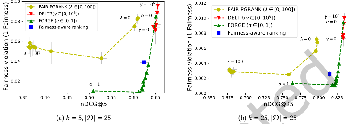
Fig. 4. COMPAS data with FeatNet as base-ranker — average nDCG vs. average 1 – fairness at intermediate and maximal cutoff k on test data. Variance is shown in gray.
