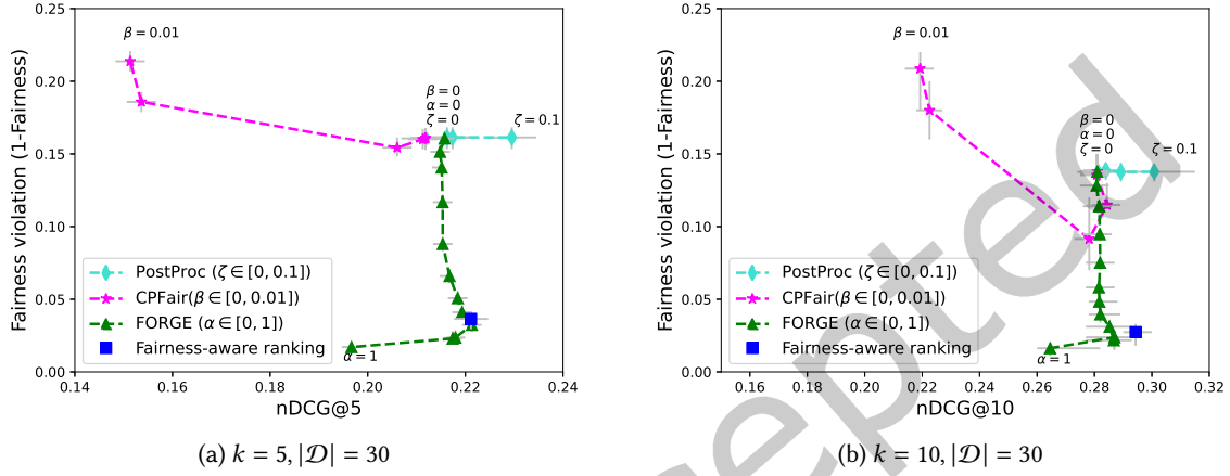
Fig. 7. Epinion data with VAE CF as base-ranker— average nDCG vs. average 1 - \text{fairness} at k = 5 , and k = 10 on test data. Variance is shown in gray
