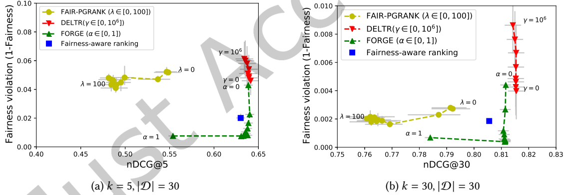
Fig. 5. MovieLens100K data with FeatNet as base-ranker— average nDCG vs. average 1 – fairness at intermediate and maximal cutoff k on test data. Variance is shown in gray.
