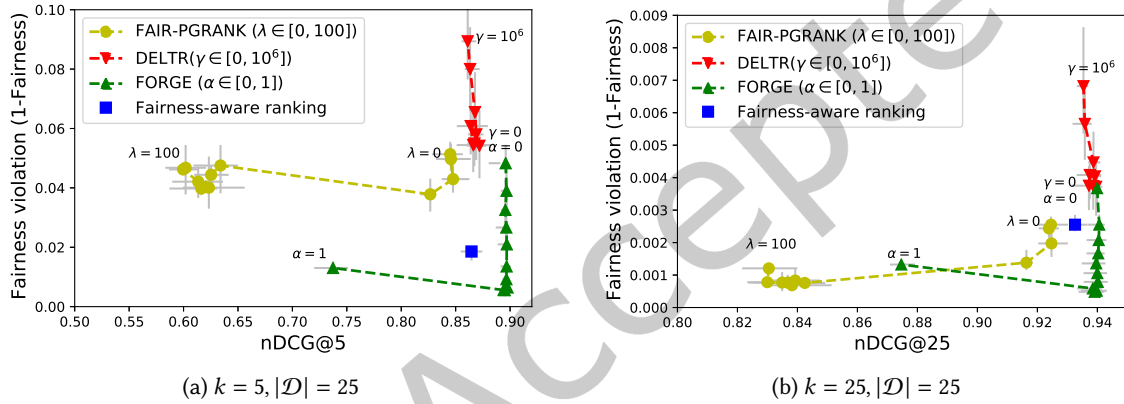
Fig. 3. German Credit data with FeatNet as base-ranker— average nDCG vs. average 1 - \text{fairness} at intermediate and maximal cutoff k on test data. Variance is shown in gray.
