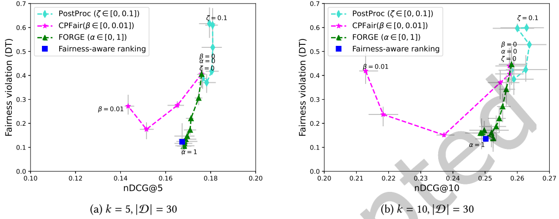
Fig. 10. MovieLens100K data with VAEF as base-ranker— average nDCG vs. average disparate treatment (DT) at k=5 , and k=10 on test data. Variance is shown in gray.
