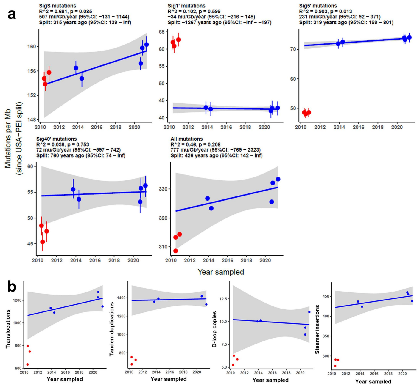
Extended Data Fig. 5 | Mutations versus sampling date. (a) Mutations attributed to each mutational signature versus sampling date for MarBTN samples. SNVs found in healthy clams, all BTN samples, or LOH regions are excluded prior to analysis to remove founder variants. Results from linear regression of USA samples ( n = 5 ) are shown above each plot, including R squared, p value, mutation rate estimate and the corresponding x -intercept (indicating date the two sub-lineages diverged from one another). PEI samples ( n = 3 ) are included on plots to compare relative mutation counts attributed to each signature but are not included in the linear regression. It is apparent that sig1' mutation counts are higher in PEI, while sig5' and sig40 mutations are higher in USA. SigS mutations in PEI line up well with the USA sample
