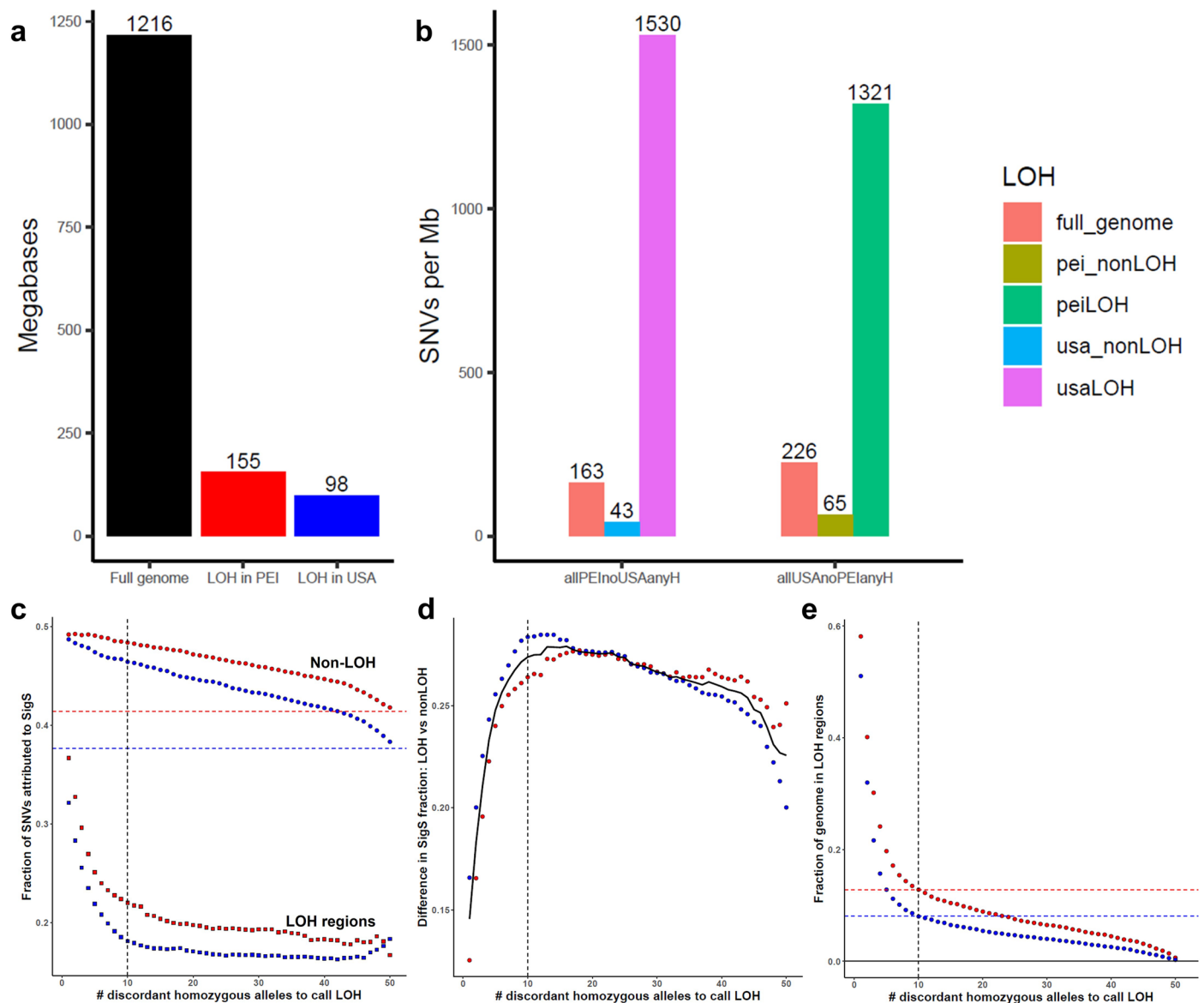
Extended Data Fig. 2 | Loss of heterozygosity regions have sub-lineage-specific founder variants. (a) Comparative sizes of the assembled genome and the fractions called as LOH in the PEI (red) and USA (blue) sub-lineages. (b) SNV density of sub-lineage-specific founder variants (variants found in a healthy clam and all individuals of one sub-lineage but none in the other sub-lineage) across the genome and LOH regions called in the other sub-lineage. Density is 36× greater for PEI mutations in USA LOH regions versus non-LOH regions and 20× greater for USA mutations in PEI LOH regions versus non-LOH regions. LOH regions were ignored for somatic mutation analysis to reduce the influence of remaining founder variants in sub-lineage specific SNVs, which should otherwise consist of somatic mutations. (c) We used various thresholds of stringency to call LOH across the genomes of each sub-lineage based on the number of shared SNVs
