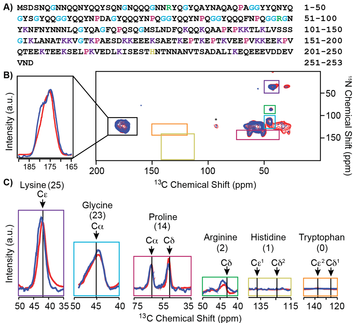
Figure 5. Specific detection of isolated sites in Sup35NM in cellular milieu. (A) Protein sequence of Sup35NM. Lysines (purple), glycines (blue), prolines (pink), arginines (green) and histadine (yellow) are highlighted. (B) Two-dimensional ^{15}\text{N} - ^{13}\text{C} correlation spectra (zTEDOR). Uniformly labeled Sup35NM in protonated, natural abundance strong [\text{PSI}^+] yeast lysate (blue) with 85% protonated buffer and 15% d_8 -glycerol with 5 mM AMUPol, n=1280 , acquisition time = 23 hours, \varepsilon=72 . Purified amyloid fibers (red) with 10% protonation, 60% ^{13}\text{C} depleted d_8 -glycerol with 10 mM AMUPol, n=128 , acquisition time = 2.5 hours \varepsilon=44 . Data were collected at 600 MHz with 12.5 kHz MAS at 104 K with a recycle of 4 seconds. Asterisks indicate spinning side bands. (C) Projections of regions of the zTEDOR for amino acids with unique chemical
