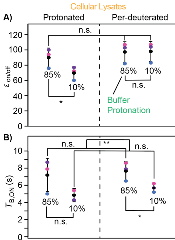
Figure 2. DNP performance is maintained in protonated DNP matrix conditions for cellular lysate samples using AMUPol. DNP sample buffer protonation scheme is marked with 85% or 10%. DNP cellular lysate protonation scheme is marked with protonated (100%) or per-deuterated (50%). Samples from the same data sets are indicated by color (pink, purple and blue). Average and standard deviations are shown in black. Black lines indicate results of paired student t -tests. (A) DNP enhancement ( \epsilon_{on/off} ) of cellular lysate samples measured by the ratio of on/off microwaves signal of the ^{13}\text{C} -CP signal at the carbonyl. (B) Build-up time values derived from ^1\text{H} -saturation recovery experiments fit to a stretched exponential function at the carbonyl are dependent upon the protonation of the buffer. Samples contain 15% d_8 -glycerol. Brackets indicate results of paired two-tailed homoscedastic student's t -tests (n.s. p > 0.05 , * p < 0.05 , ** p < 0.01 ).
