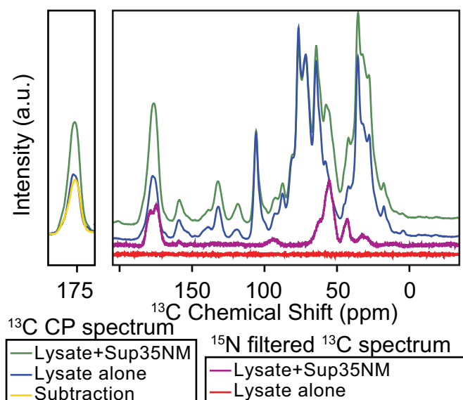
Figure 4: The protein of interest and naturally abundant cellular lysates have predictable magnitudes of contribution to the spectrum. The ^{13}\text{C} spectra of natural abundance lysate alone (blue) has many signals while the ^{15}\text{N} filtered ^{13}\text{C} spectra has none (red). The ^{13}\text{C} spectra of 25
