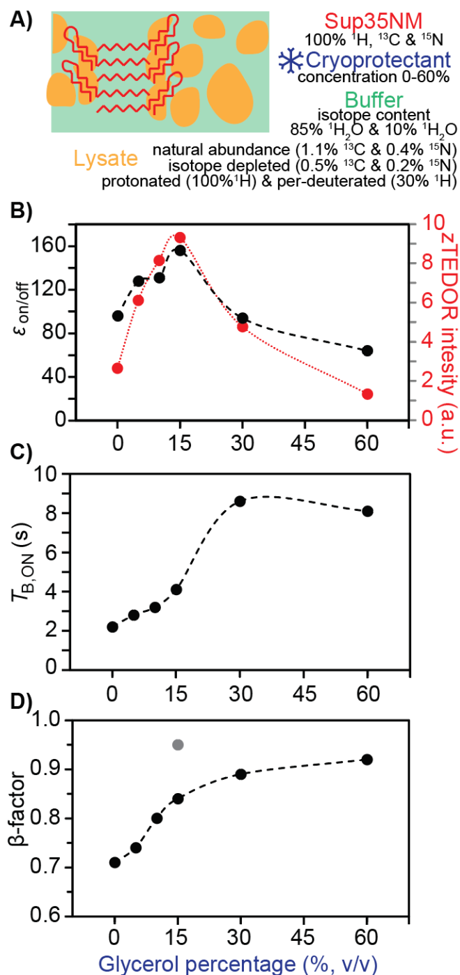
Figure 1 Lower cryoprotectant percentages result in better DNP performance of dilute proteins in pelleted cellular lysates. A) Sup35NM (red) is diluted in a matrix composed of cryoprotectant (blue), solvent in the buffer (green) and cellular components (yellow), all of which can have
