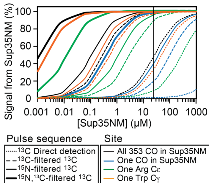
Figure 3: Specificity for the isotopically enriched protein of interest diluted in natural abundance cellular milieu depends upon the concentration of the protein of interest, the selectivity of the pulse sequence, and the degeneracy of the chemical shift of the site. The percent of the signal that is derived from isotopically enriched Sup35NM rather than from the natural molecules in the cellular milieu increases as the concentration of Sup35NM added to the sample increases. When Sup35NM is present at 25 \mu M (vertical line), the signal from all the carbonyl carbons in Sup35NM and from the cellular milieu is calculated to be of equal magnitude (dotted black line). Selection for sites with an adjacent isotopically labeled carbon (dashed lines) or nitrogen (solid lines) decreases the contribution from the cellular milieu by two orders of magnitude. Selection for a site through two adjacent isotopically labeled sites (thick lines) decreases the contribution from the cellular milieu by four orders of magnitude. All amino acids have at least one carbonyl moiety so specific detection of a single labeled CO site requires high concentrations and/or very selective pulse sequences (blue lines). Single sites in less abundant amino acids and/or in unique chemical moieties can be specifically detected at lower concentrations. About 5% of the amino acids in yeast are Arg (green) while only 1% are Trp (orange). With the use of highly selective pulse sequences these sites can be specifically detected (>98%) at 100 nM or lower concentrations.
