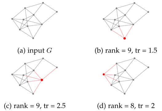
Fig. 2. Controllability metrics vary with leader selection
