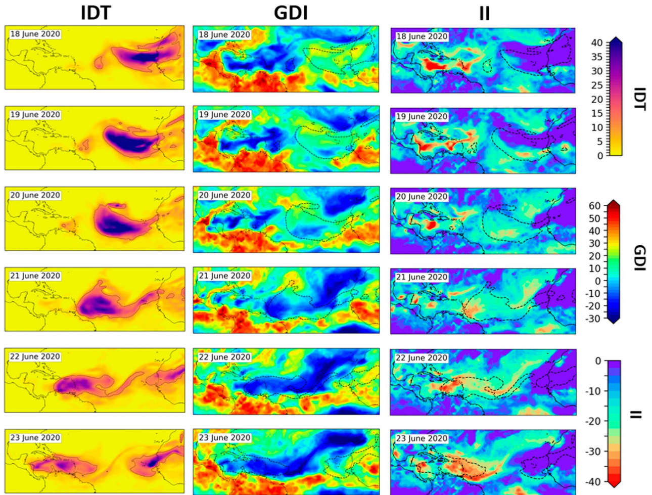
Figure 7. Daily IDT, GDI, and II between 18 and 23 June 2020 coinciding with a significant Saharan dust outbreak. The 10\text{-g m}^{-1}\text{ s}^{-1} IDT contour is drawn in all three variables as a black dashed line. All days above were grouped to node 12 except for 18 and 23 June when the IDT distributions were briefly sorted to nodes 9 and 10, respectively.
