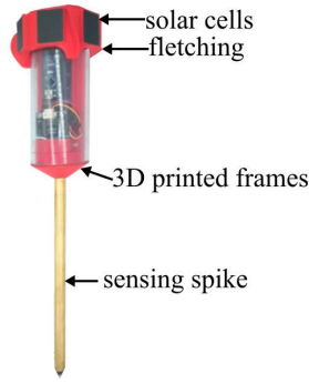
FIGURE 2. The UAV deployable sensor package.
