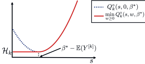
Figure 4. Q_k^\circ(s, 0, \beta^*) versus \min_{w \geq 0} Q_k^\circ(s, w, \beta^*)
