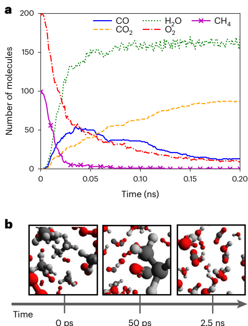
Fig. 6 | Methane combustion simulation results for ANI-1xnr. a , A tracking plot of \text{O}_2 , \text{CH}_4 and major products ( \text{CO} , \text{CO}_2 and \text{H}_2\text{O} ). The tracking plot for the full simulation is provided as Supplementary Fig. 3. b , Snapshots of initial reactants, intermediate species and final products. Both the tracking plot and the snapshots confirm that ANI-1xnr predicts qualitatively reasonable reactive chemistry for this system. However, ANI-1xnr is markedly more reactive than the application-specific MLIP in the literature 24 .
