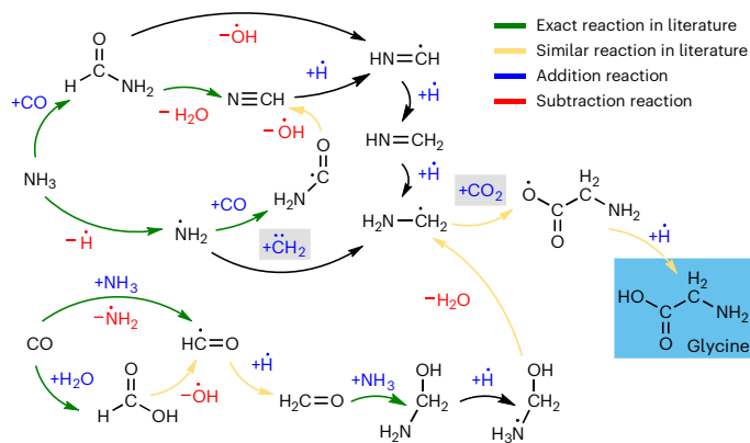
Fig. 7 | Miller experiment simulation results for ANI-1xnr. The reaction pathways discovered by ANI-1xnr in a Miller experiment simulation for the formation of glycine from small-molecule species (for example, \text{NH}_3 , \text{CO} , \text{H}_2\text{O} , \text{H}_2 and \text{CH}_4 ). The green arrows denote reactions previously identified by Wang et al. or Saitta and Saija. The orange arrows denote reactions that have a similar reaction in Wang et al. or Saitta and Saija. The majority of reactions have been previously reported in the literature, confirming the validity of the ANI-1xnr mechanism. Three-dimensional snapshots extracted from the MD simulation trajectory are reported in Extended Data Fig. 6, further confirming that the reaction pathways are physically meaningful. Note that +H does not necessarily signify a free hydrogen atom, +H is short-hand for a proton donor, for example, \text{NH}_4 , \text{NH}_3 , \text{CHO} , \text{CHNO} , \text{H}_3\text{O} or \text{H}_2\text{O} . Likewise, -H does not necessarily signify dissociation of a hydrogen atom. -H is short-hand for a proton acceptor, for example, \text{NH}_2 , \text{CO} , \text{CNO} , \text{H}_2\text{O} or \text{OH} . The boxes encapsulate the key intermediates, carbon dioxide ( \text{CO}_2 ) and methylene ( \text{CH}_2 ). The novel pathways to form these key intermediates are reported in Extended Data Fig. 7. The depiction of bond orders and radical species is based simply on chemical intuition, since ANI-1xnr does not provide explicit bonding, orbital or electronic information (for an alternative interpretation of this mechanism involving ionic species, see Extended Data Fig. 8).
