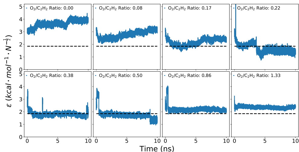
Extended Data Fig. 1 | ANI-1xnr uncertainty for all eight \text{O}_2/\text{C}_2\text{H}_2 ratios in graphene ring formation simulations. Uncertainty ( \varepsilon ) is computed as ensemble standard deviation in energy normalized by the square-root of number atoms. Dashed black line corresponds to AL energy threshold of 1.85 \text{ kcal mol}^{-1} \text{ N}^{-1/2} . The MLIP uncertainty is fairly constant and approximately equal to the AL energy threshold through nearly the entire simulation (with only a few snapshots as exceptions). The relatively low and constant uncertainty confirms that each system is well-modeled by our MLIP. It is also interesting that the MLIP uncertainty decreases with increasing \text{O}_2/\text{C}_2\text{H}_2 ratio, suggesting that ANI-1xnr is most confident under a higher \text{O}_2/\text{C}_2\text{H}_2 ratio. The reason for such a tendency is
