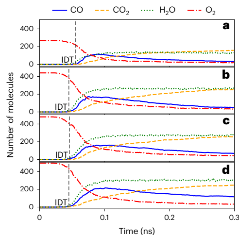
Fig. 5 | Biofuel additive simulation results for ANI-1xnr. a–d , Tracking plots of O_2 and major products (CO, CO_2 and H_2O ) for the following biofuel simulations: biofuel + O_2 ( a ), biofuel + O_2 with ethanol additive ( b ), biofuel + O_2 with 2-butanol additive ( c ) and biofuel + O_2 with MTBE additive ( d ). IDT is defined as the average time that at least five molecules of CO, CO_2 and H_2O are produced (Supplementary Fig. 1). IDT is significantly decreased for each additive in comparison with the clean biofuel. For tracking plots including the entire 2 ns simulation, see Extended Data Fig. 2.
