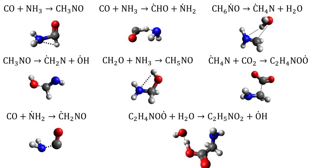
Extended Data Fig. 6 | Three-dimensional structures of reactions discovered by ANI-1xnr in Miller experiment simulation. Structures are snapshots extracted directly from the MD simulation trajectory, providing visual confirmation that the reaction pathways are physically meaningful.
