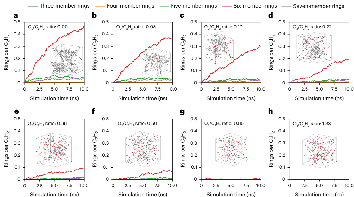
Fig. 4 | Effect of oxygen on graphene ring formation simulation results for ANI-1xnr. a–h , A comparison of three-, four-, five-, six- and seven-membered ring formation for different ratios of O_2/C_2H_2 : 0.00 ( a ), 0.08 ( b ), 0.17 ( c ), 0.22 ( d ), 0.38 ( e ), 0.50 ( f ), 0.86 ( g ) and 1.33 ( h ). ANI-1xnr predicts six-membered ring formation for O_2/C_2H_2 ratios less than 0.50, in closer agreement with experimental data
