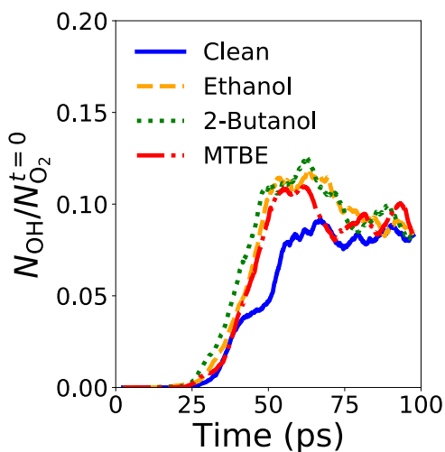
Extended Data Fig. 3 | Comparison of normalized production rate of OH for biofuel additive simulations. Number of OH species ( N_{\text{OH}} ) is normalized by the initial number of \text{O}_2 molecules ( N_{\text{O}_2}^{t=0} ). In comparison to the pure biofuel, all three systems with additives have a higher and earlier peak in OH radical, when normalized by the initial amount of \text{O}_2 . The enhancement in OH production for ethanol is intuitive since ethanol contains a hydroxyl group with a similar bond
