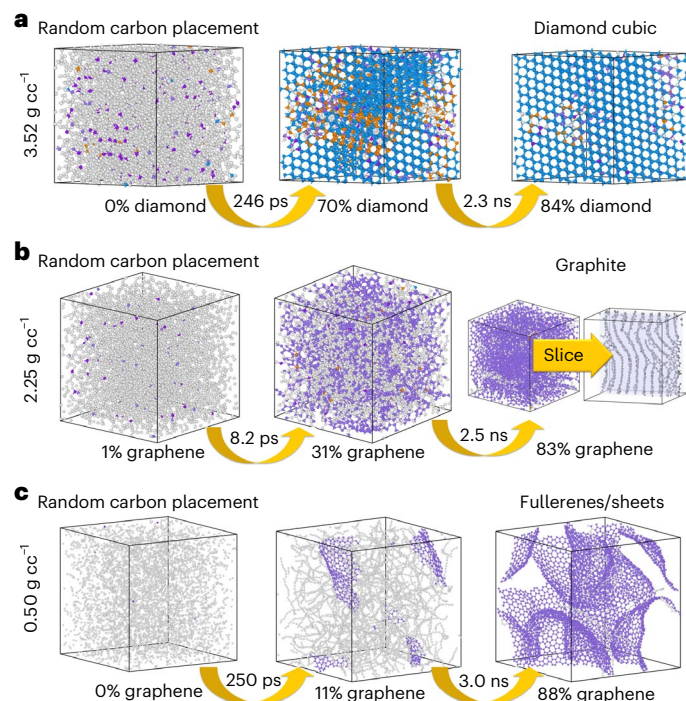
Fig. 3 | Carbon solid-phase nucleation simulation results for ANI-1xnr.
