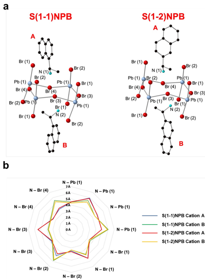
Figure 7. (a) Schematic of cation A and B in S(1-1)NPB and S(1-2)NPB for calculation of N-Pb/Br distances (Table S7 and Table S8). Blue, red, black, and turquoise spheres denote Pb, Br, C, and N atoms, respectively. The obtained data for S(1-1)NPB is derived from our previously published work. 45 (b) Radar chart of the N-Pb/Br distances of type A and B cations in S(1-1)NPB and S(1-2)NPB. Blue and green lines denote the cation A and B of S(1-1)NPB, respectively. Red and yellow lines indicate the cation A and B of S(1-2)NPB, respectively.
