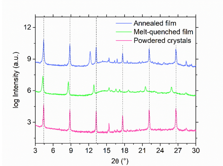
Figure 3. Logarithmic scale XRD profiles of S(1-2)NPB powdered crystals, melt-quenched film, and annealed film. The spectra of the films are taken under an overlayer of Kapton as a part of the melt processing to avoid loss of material upon heating. The (00l) family of crystalline peaks for the powdered crystals are shown by vertical dotted black lines as a guide to the eyes. The vertical axis is only for representation of scale of magnitude, i.e., the curves are vertically offset for clarity.
