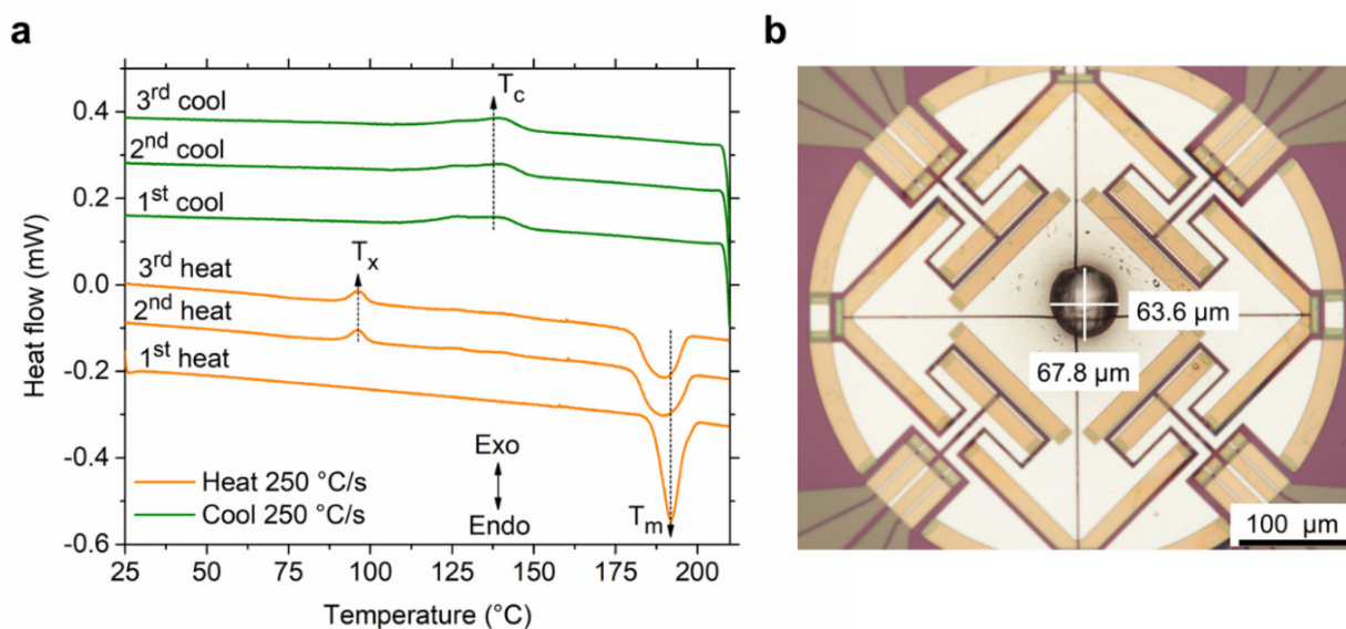
Figure 4. (a) Three iterations of ultrafast calorimetric (Flash-DSC) measurement performed on a single crystal of S(1-2)NPB. The first heating cycle (250 °C/s) shows a sharp initial melting ( T_m ) step. Cooling the formed melt (at the same ramp rate) results in partial glass formation and partial melt crystallization ( T_c ). During the second heating cycle, cold crystallization ( T_x ) of the partially formed glass is observed with subsequent melting ( T_m ) of the fully crystallized volume. A third iteration is provided to show consistency of the thermal features. The vertical axis is only for representation of scale of magnitude, i.e., the curves are vertically offset for clarity. (b) Optical microscopy image of the crystallized S(1-2)NPB sample (diameter of ~65 μm) mounted on UFS-1 chip under silicone oil. The image was captured at the conclusion of all the measurements conducted on the sample.
