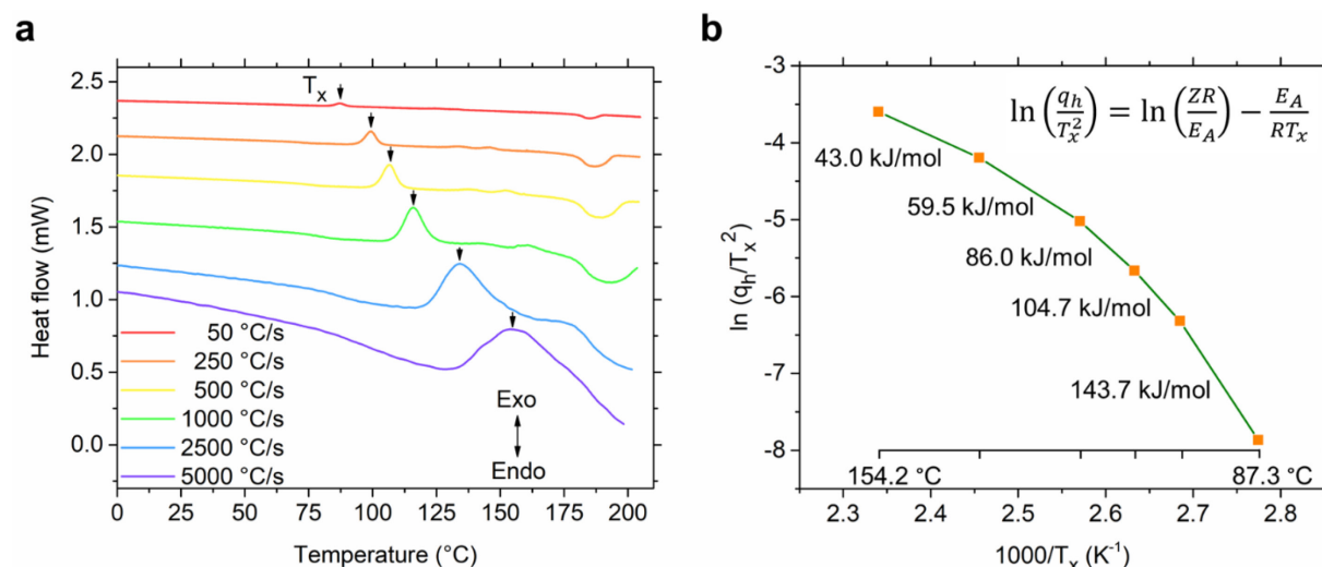
Figure 6. Kinetics of glass crystallization. (a) Heating curves of S(1-2)NPB obtained at different ramp rates after the glass formation step (melt quenching at CCR, see Figure S5). The shift in the cold crystallization peak ( T_x , shown by arrow) with increasing heating rate suggests the kinetic nature of glass-crystallization behavior. The vertical axis is only for representation of scale of magnitude, i.e., the curves are vertically offset for clarity. (b) The shifts in T_x values are used in constructing a Kissinger plot to determine the activation energy of glass crystallization ( E_A , slope of the curve). The slope of the plot shows a large deviation from a linear trend over the course of change in heating ramp rates (50 °C/s – 5000 °C/s), revealing breakdown of Arrhenius behavior.
