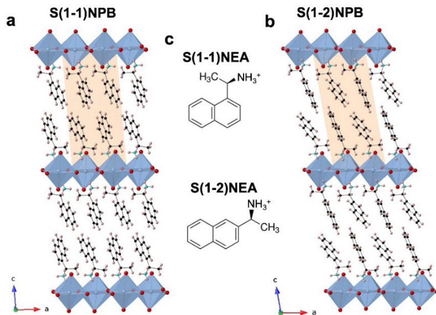
Figure 1. Schematic single-crystal structures of (a) S(1-1)NPB and (b) S(1-2)NPB. Unit cells in a-b are indicated by shaded parallelograms. (c) The molecular structure of S(1-1)NEA and S(1-2)NEA cations. The different molecular structures induce the characteristic orientations of organic cations within the 2D HOIPs. Blue, red, black, turquoise, and beige spheres denote Pb, Br, C, N, and H atoms, respectively.
