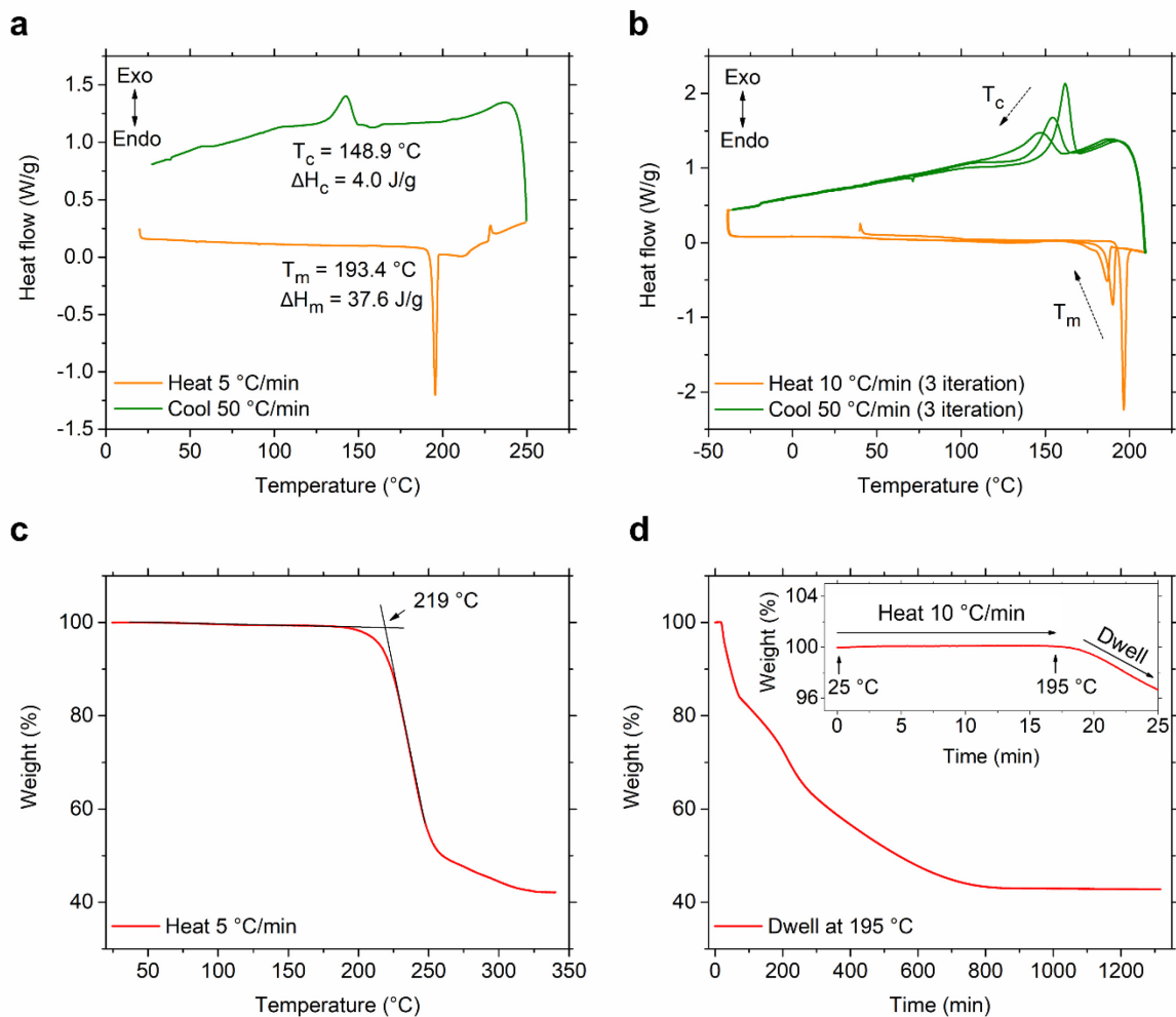
Figure 2. Conventional differential scanning calorimetry (DSC) analysis of the S(1-2)NPB sample. (a) The heating and cooling DSC scans depict complete melting of the sample, accompanied by partial melt crystallization with distinct temperatures ( T_m , T_c ) and corresponding enthalpies ( \Delta H_m , \Delta H_c ). (b) Iterative heating and cooling DSC cycles reveal a decrease in temperature and enthalpies of melting and crystallization as a function of iteration. No glass formation or cold crystallization behavior is observed over an extended temperature range (lower end). (c) Thermogravimetric analysis (TGA) of the S(1-2)NPB crystals on continuous heating and (d) isothermal hold (dwell) at 195\text{ °C} ( >T_m ) over multiple hours. The weight change to \sim 43\% at
