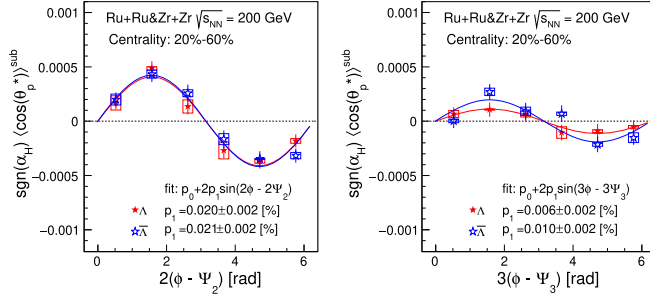
FIG. 2. \langle \cos \theta_p^* \rangle^{\text{sub}} of \Lambda and \bar{\Lambda} as a function of hyperon azimuthal angle relative to the second- (left panel) and the third-order (right panel) event planes, n(\phi - \Psi_n) , in 20%–60% central isobar collisions at \sqrt{s_{NN}} = 200 GeV. The sign of the data for \bar{\Lambda} is flipped as indicated by \text{sgn}(\alpha_H) . The solid lines are fit functions used to extract the parameters indicated in the label where p_1 corresponds to the n th-order Fourier sine coefficient. Note that the results presented in these figures are not corrected for the event plane resolution.
